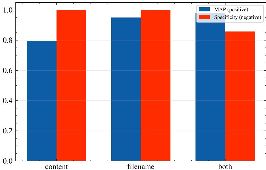
Accuracy by scope
