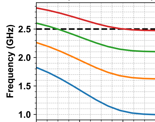
Slow (SS 125°C, 0.9 V)
