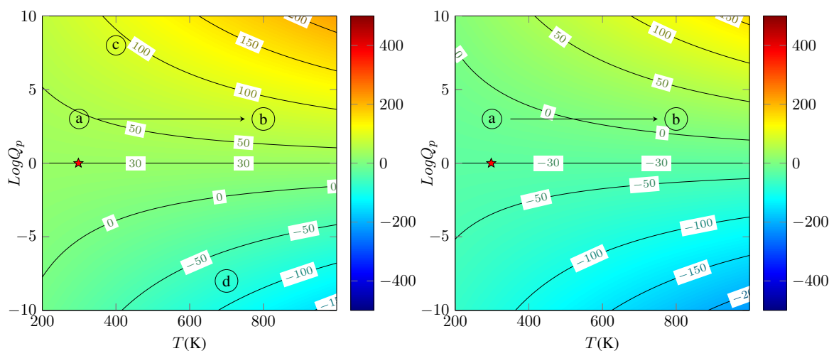
Figure 7.3 Gibbs free energy 2D plots displaying contour lines for different pressure and temperature conditions for an endergonic (Left Panel) and an exergonic (Right Panel) reaction. The star sign indicated the standard pressure and temperature conditions. The equilibrium isoline corresponds to \Delta G_R = 0 . The same heating experiment is carried out with both reactions. Increasing the temperature until reaching the conditions labeled as b does not affect the spontaneity of the reaction on the left, whereas it impedes the reaction on the right, which is now non-spontaneous under b conditions ( \Delta G_R > 0 ).
