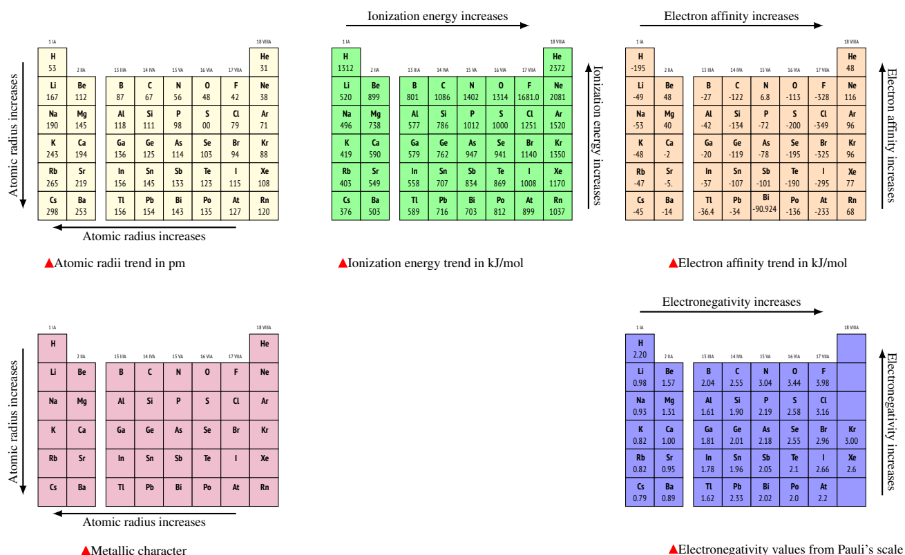
Figure ?? Periodic properties across the periodic table
