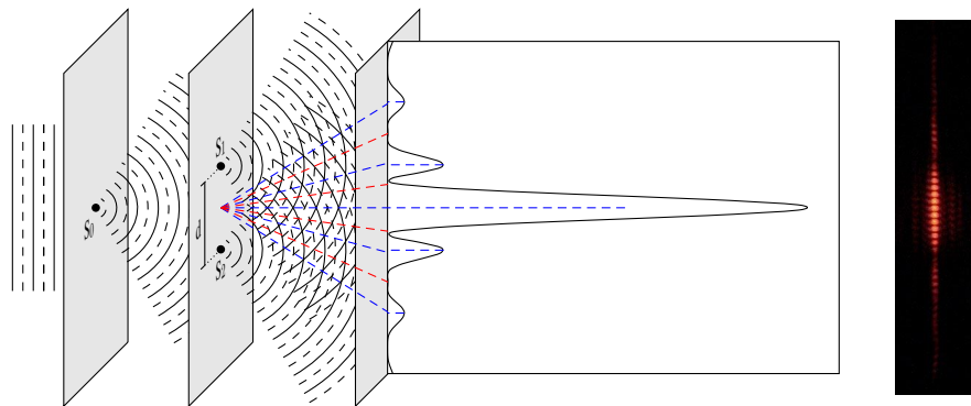
Figure ?? The double-slit experiment demonstrating the wave nature of light. Using one slit leads to a single bright spot. Using two slits leads to a set of patterns of light and darkness resulting from the interference of light. Red lines represent destructive interference whereas blue lines represent constructive interferences.
