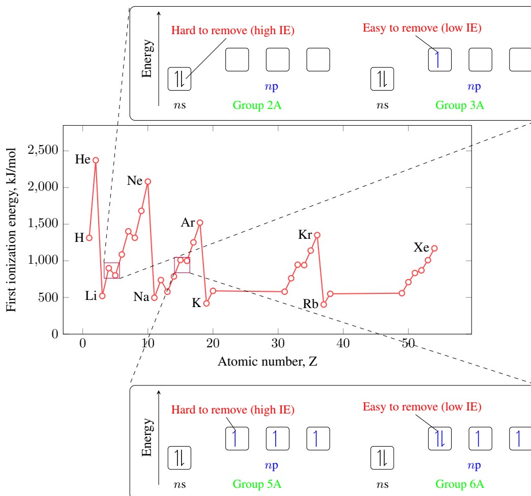
Figure ?? Ionization energy graphed with respect to the atomic number
