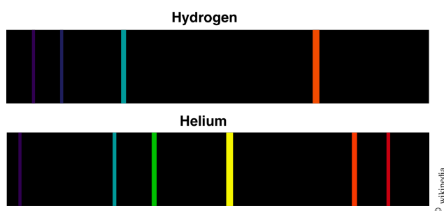
Figure ?? Atomic spectrum of two atoms showing the lines corresponding to the visible.
