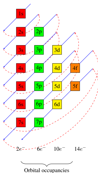
Figure ?? Orbital filling order.
