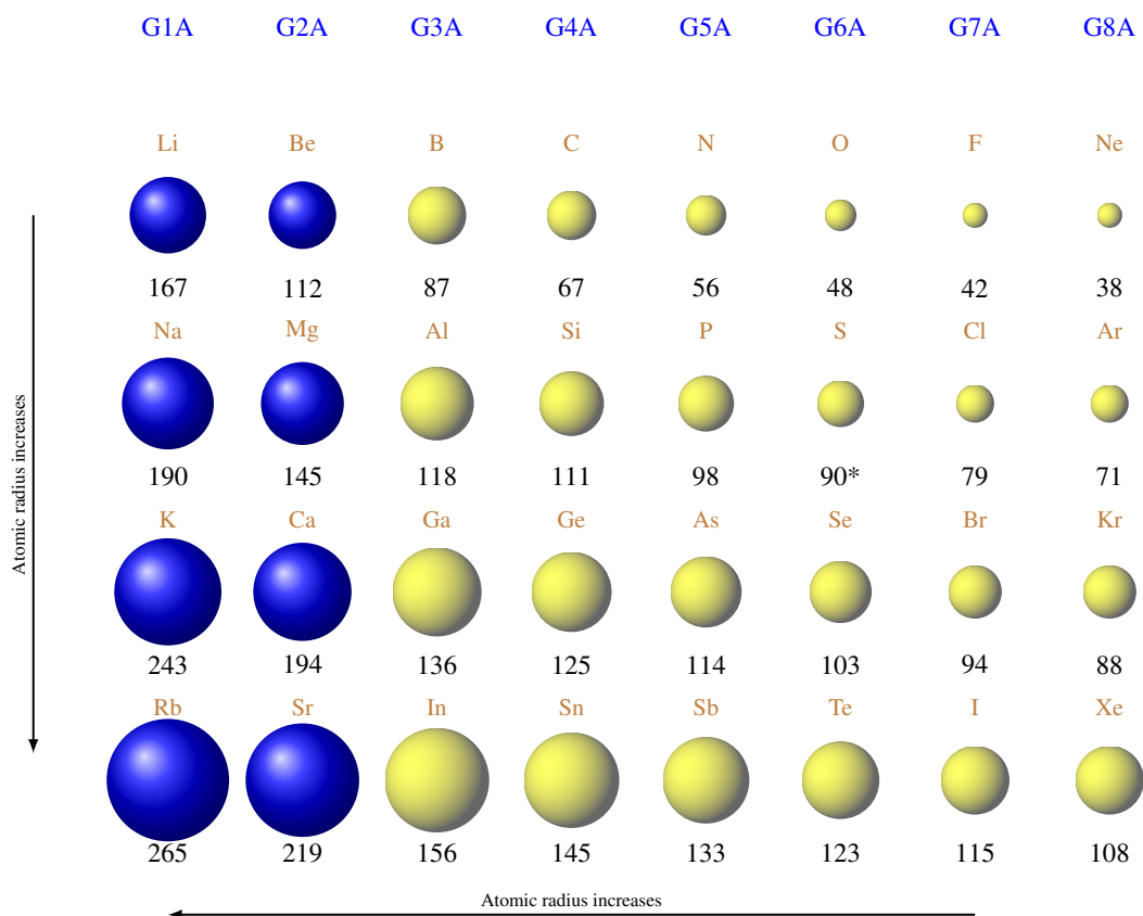
Figure ?? Change of atomic radius (calculated values given in pm) across the periodic table. The value with * was estimated
