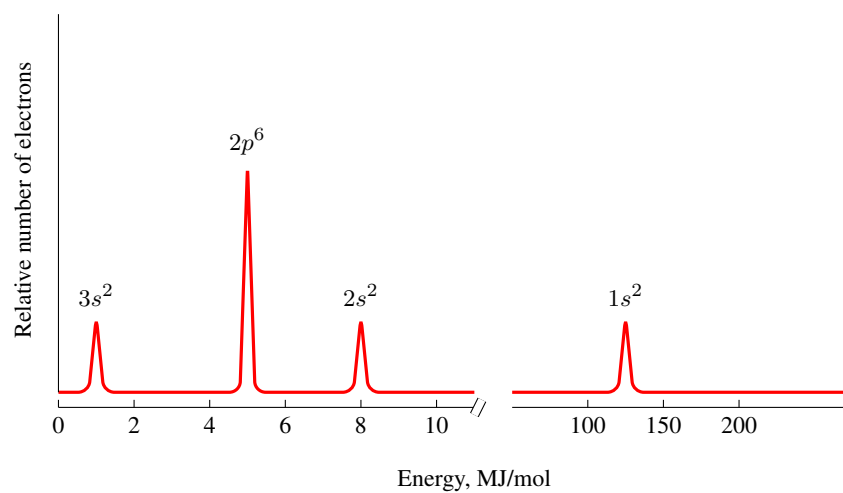
Figure ?? Photoelectron spectrum (PES) of Magnesium
