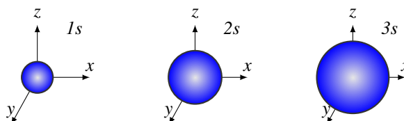
Figure ?? Surface plots of three s orbitals.
