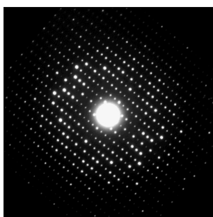
Figure ?? Diffraction patterns produced by light and by matter
