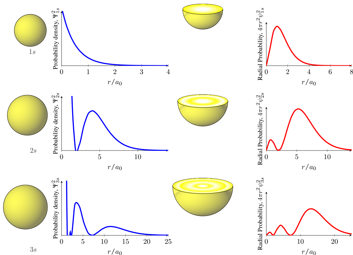
Figure ?? Three different representations of the s atomic orbitals of hydrogen: (left) boundary surface plots, (center) probability density plots (the orbital squared) with a sliced 3D surface plots, and (right) radial probability function. The value of a_0 , called Bohr's radius, is 52.9pm. The yellow circles inside the sliced 3D surface plots represent the orbital nodes.
