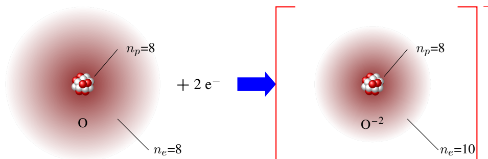
Figure ?? The formation of an oxygen anion.
