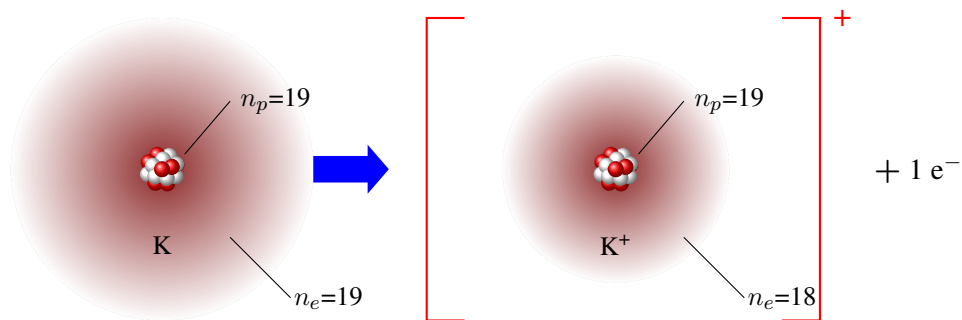
Figure ?? The formation of a potassium cation
