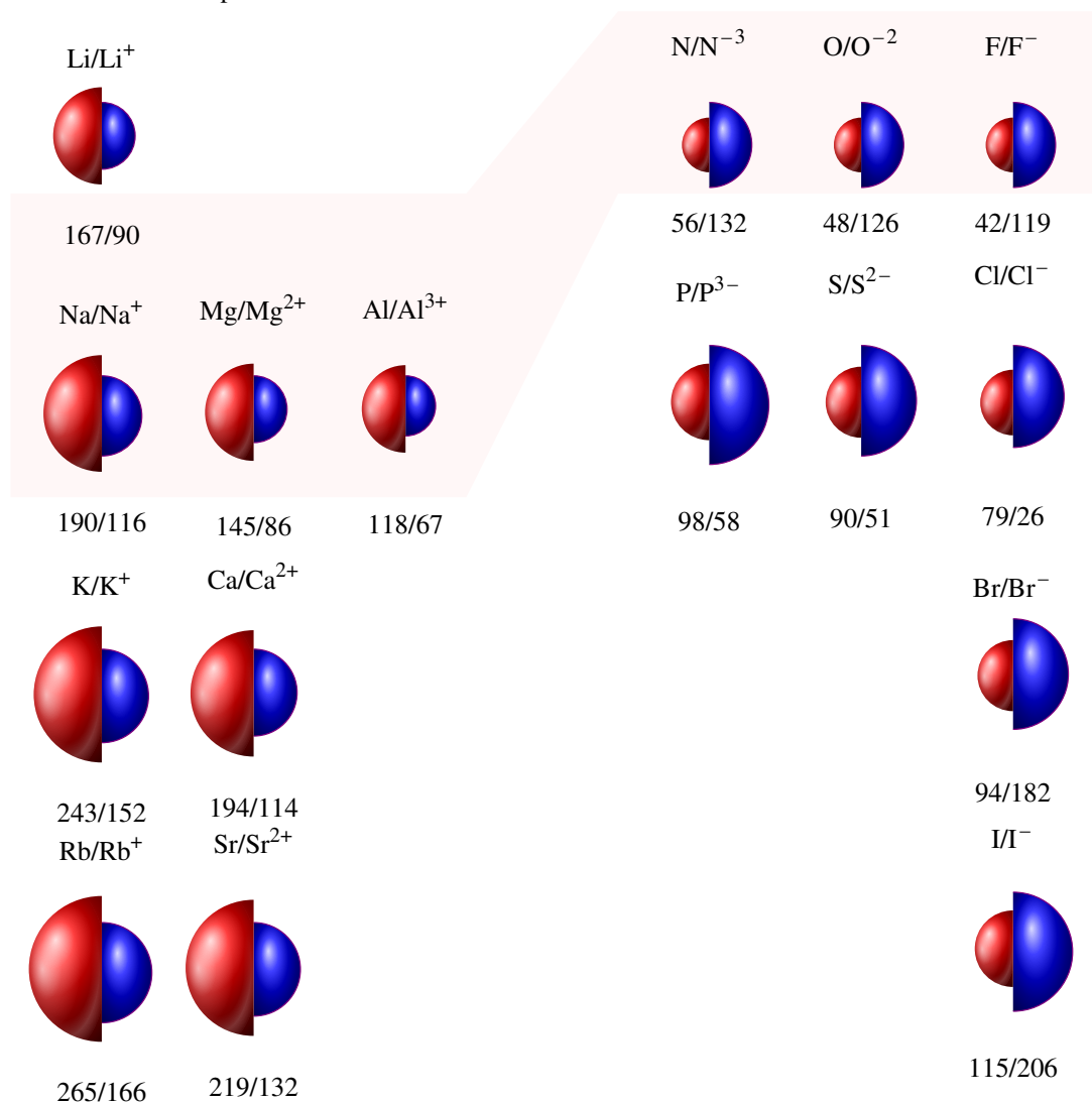
Figure ?? Ionic and atomic radius in pm across the periodic table
