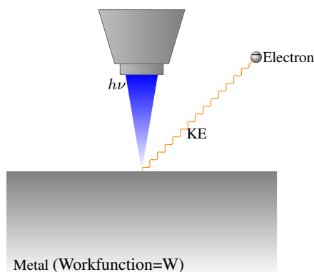
Figure ?? The photoelectric effect: when light with frequency ( \nu ) larger than a threshold irradiates a metal, electrons are ejected with a specific kinetic energy (KE) that depends on the work function ( W ) of the metal.
