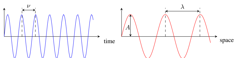
Figure ?? Properties of waves. Waves are characterized by its frequency, wavelength and amplitude and in the vacuum they travel at the speed of light.
