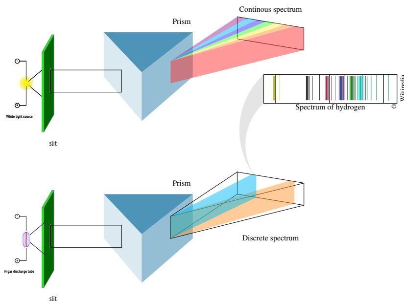
Figure ?? The spectrum of hydrogen: white light contains radiation of all colors of the visible spectrum whereas light coming from hydrogen contains a quantized series of lines.
