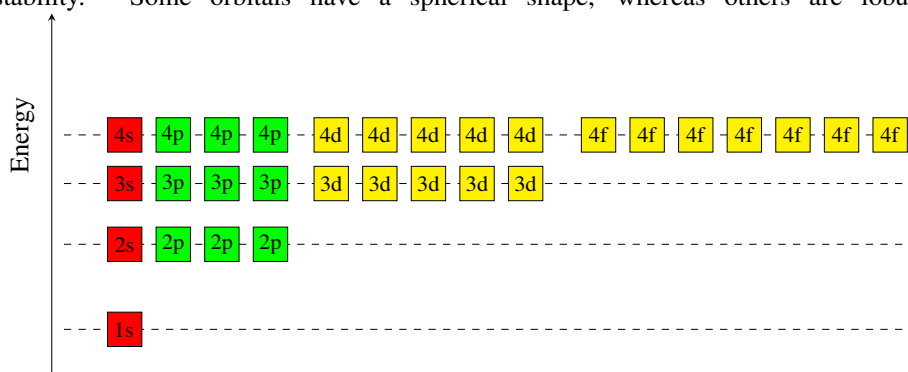
Figure ?? Energy of the different hydrogen orbitals. s orbitals have the lowest energy and hence are the most stable. Orbitals in the same shell ( 2p , 2s ) have the same energy. The larger the principal quantum number the more positive the energy, the less stable the orbital.
