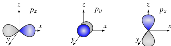
Figure ?? Surface plots of the three p orbitals.
