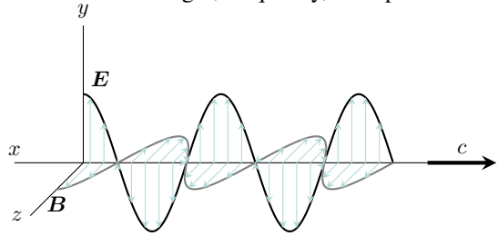
Figure ?? The electric ( E ) and magnetic ( B ) field components of an electromagnetic wave. Both fields are perpendicular.
