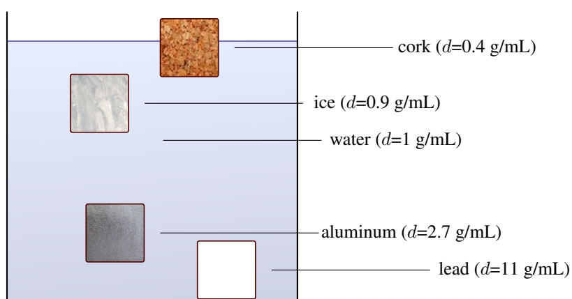
Figure ?? Objects with a larger density than water will sink whereas objects with a smaller density will float.
