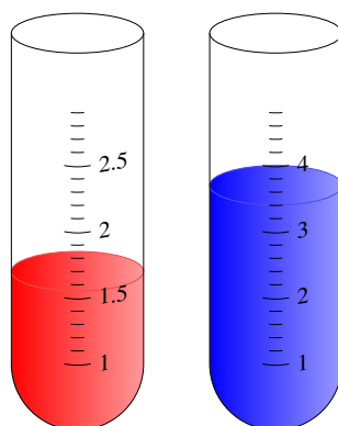
Figure ?? Two measuring devices. (Left side) The measuring device gives volumes to the hundredth place. (Right side) The measuring device gives volumes to the tenth place.
