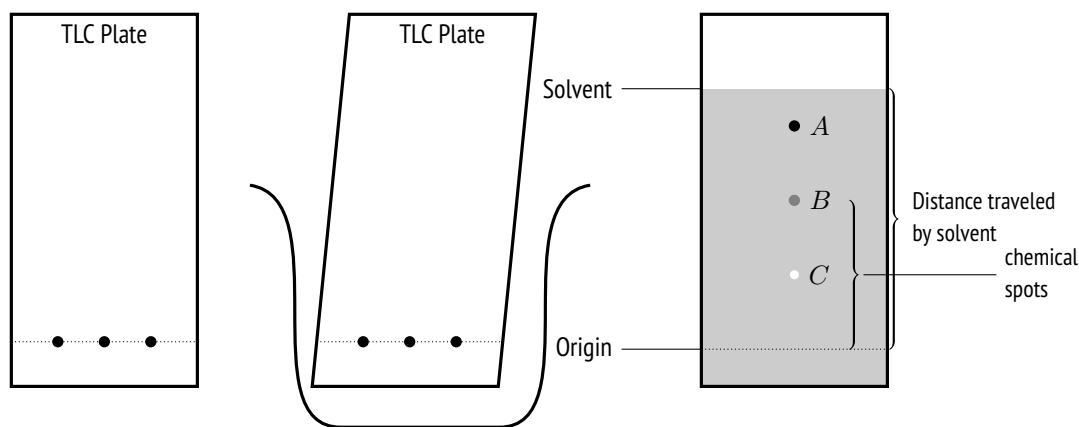
Figure ?? TLC set up. (Left) Solid phase with spots (Center) Solid phase inside a beaker containing the liquid phase (Right) Solid phase with separated mixture components.
