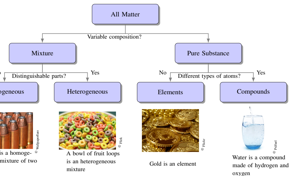
Figure ?? Classification of the matter
