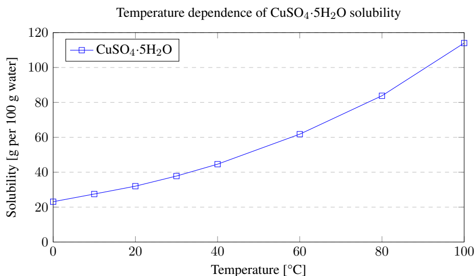
Figure ?? A graph plotting the change of solubility of a chemical with temperature.
