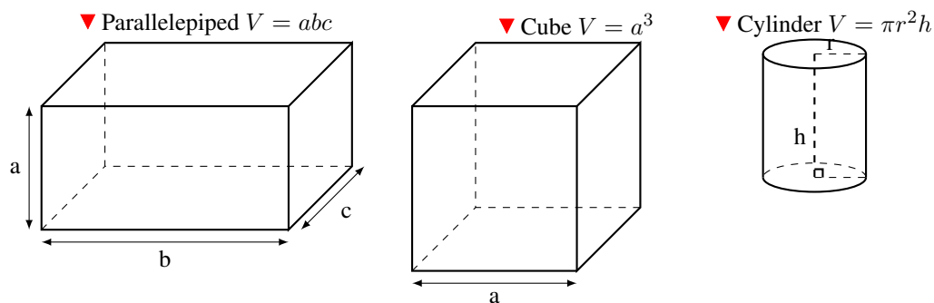
Figure ?? Volume of some objects
