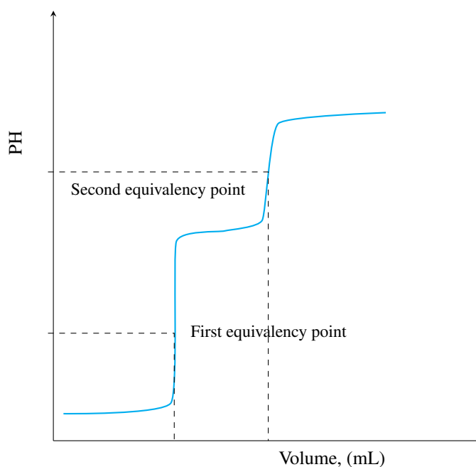
Figure 5.6 PH curve for a diprotic acid showing two equivalency points
