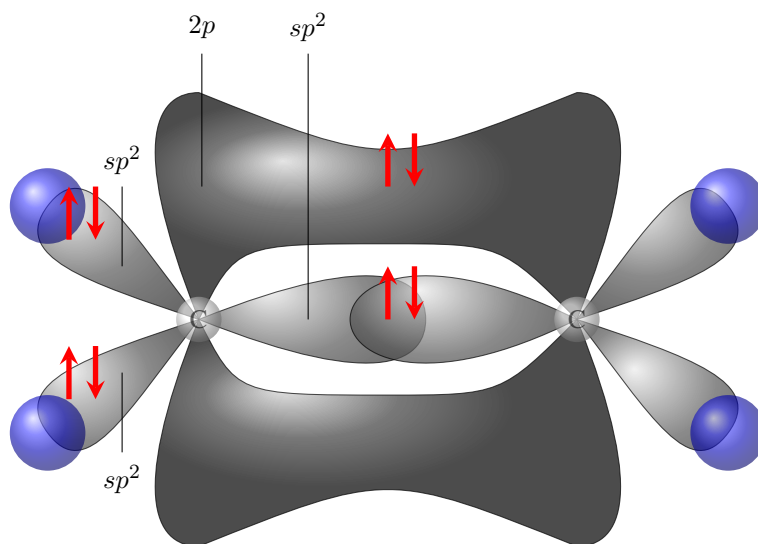
Figure ?? Bonding of ethylene in which three sp^2 hybrid orbitals and one 2p orbital populated with paired electrons. The orbitals of C (H) are represented with grey (blue) shading.
