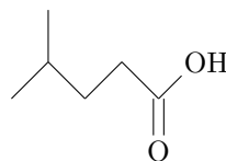
4-methylpentanoic acid
