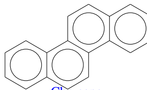
Chrysene
