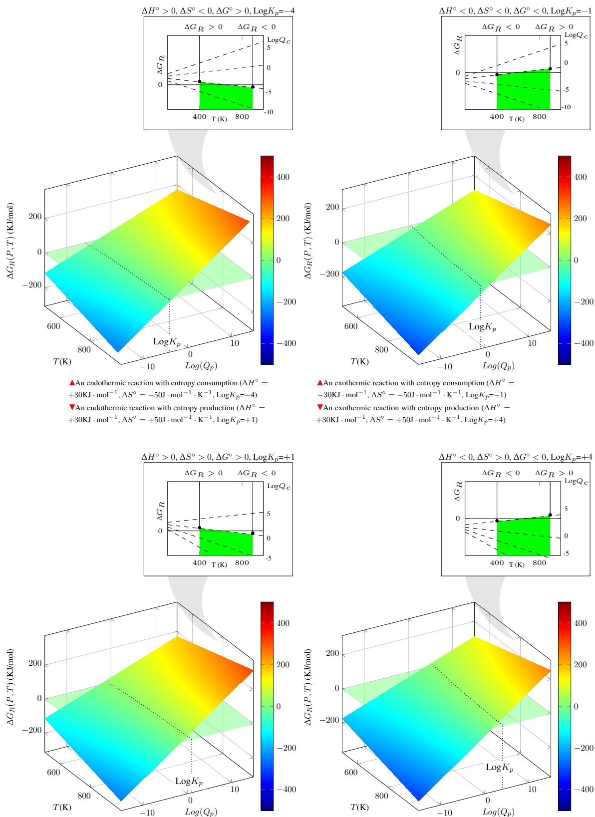
Figure 7.4 Gibbs free energy 3D plot for a set of reaction with different internal thermodynamics parameters: (Top Left) an endergonic reaction: you can increase T to favour the reaction only for pressure conditions ( \text{Log} Q_c ) lower than \Delta S/R ; (Top Right) an exergonic reaction mediated by H: you disfavour the reaction by increasing T only for pressure conditions ( \text{Log} Q_c ) higher than \Delta S/R ; (Bottom Left) an endergonic reaction mediated by S: you can increase T to favour the reaction only for pressure conditions ( \text{Log} Q_c ) lower than \Delta S/R ; (Bottom Right) an exergonic reaction mediated by both the H and S: you disfavour the reaction by increasing T only for pressure conditions ( \text{Log} Q_c ) higher than \Delta S/R ;
