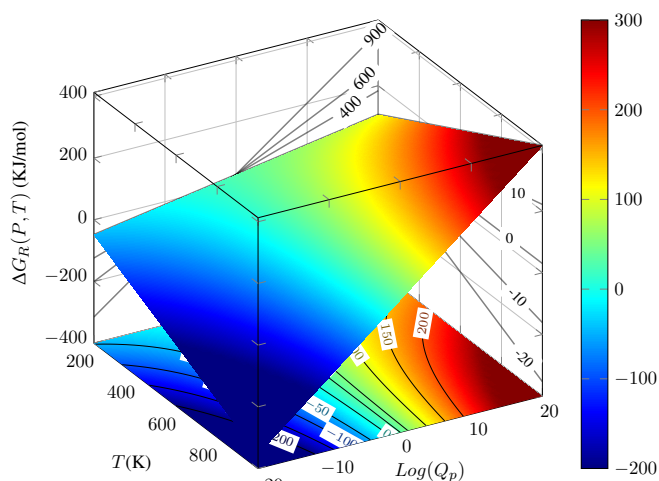
Figure 7.2 Gibbs free energy 3D plot displaying top-down projection into the \text{Log}Q_p - T bottom plane giving \Delta G isolines, into the \Delta G - T , right plane giving isobars with constant Q_p , and into the \Delta G - \text{Log}Q_p , left plane giving isotherms with constant T . The color scale is blue for negative, small \Delta G_R values, changing into red for positive, large \Delta G values.
