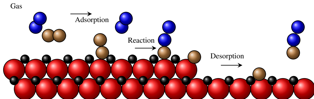
Figure 3.8 Steps in a heterogeneously catalyzed reaction
