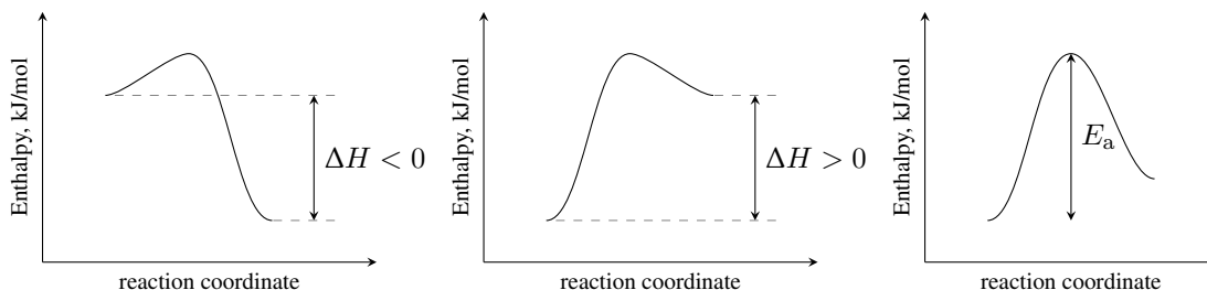
Figure 3.9 A set of reaction energy profiles displaying the energy of reaction and the activation energy: exothermic (left), endothermic (center), and endothermic (right)
