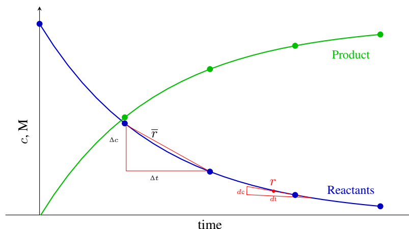
Figure 3.1 Change of the concentration of reactants and products with time showing the average and instantaneous velocity.
