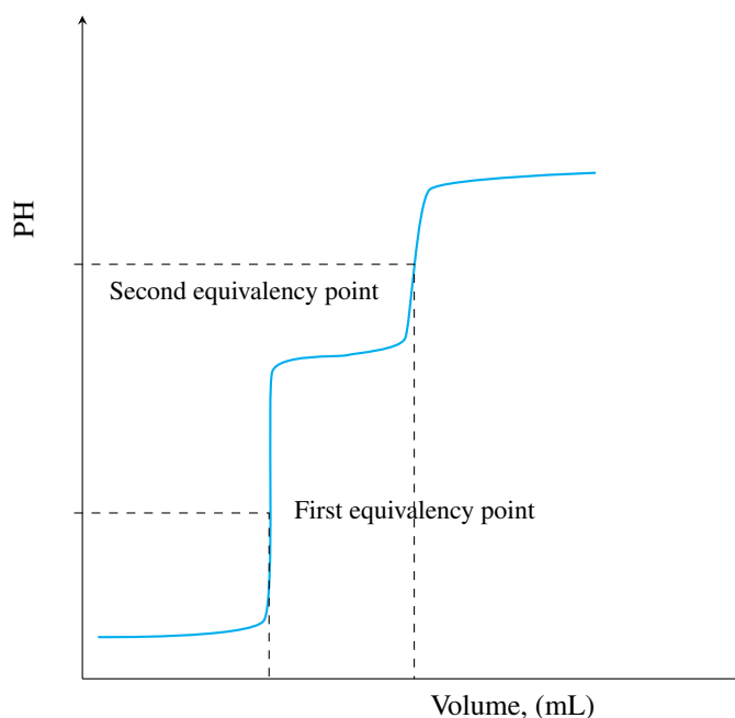
Figure ?? PH curve for a diprotic acid showing two equivalency points
