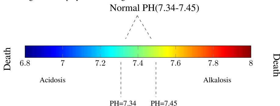
Figure ?? PH range that leads to acidosis and alkalosis
