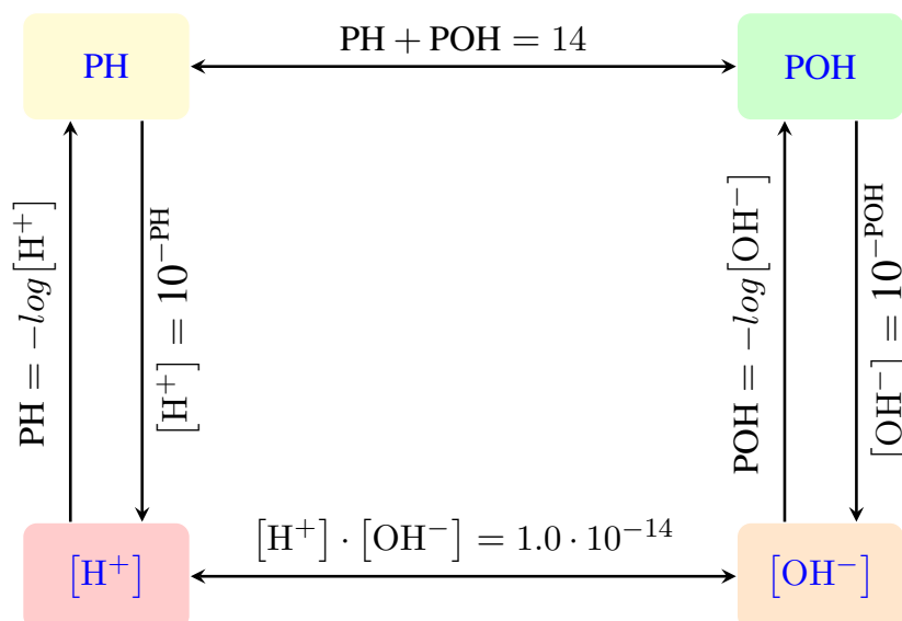
Figure ?? Diagram with formulas relating the PH, POH and the concentration of protons and hydroxyls in water.
