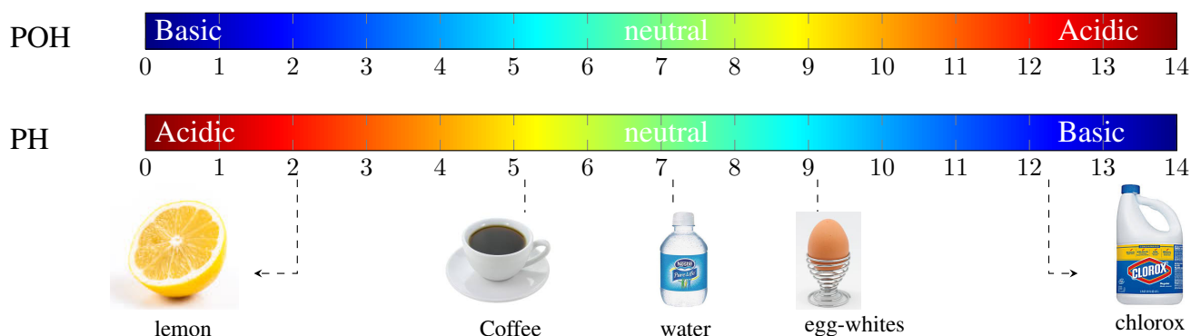
Figure ?? The PH scale
