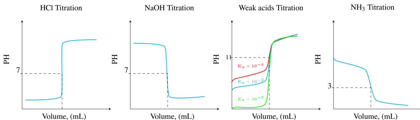
Figure ?? Different shapes of titration curves. Plateaus are flat for the PH curves of strong acids and bases, while being inclined for weak electrolytes. For weak electrolytes, plateaus are referred to as buffer areas.
