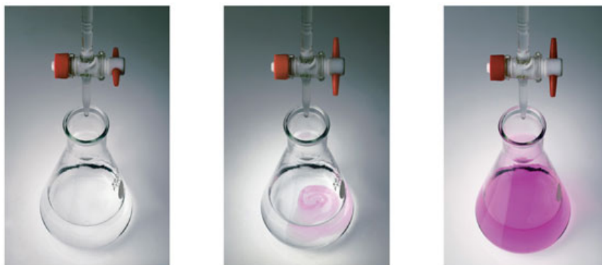
Figure ?? An acid base titration using phenolphthalein as indicator. From left to right, before, at and after the end point.
