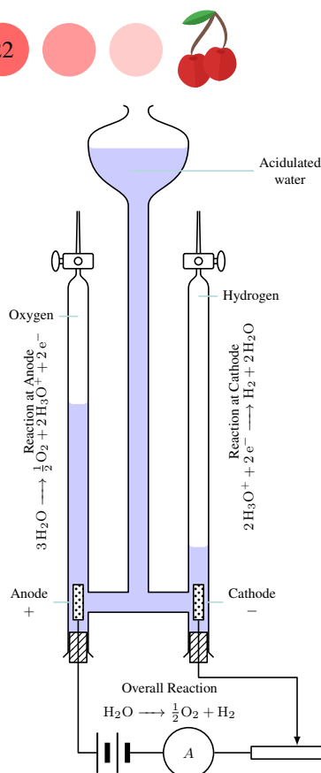
▲ Experimental set up for the electrolysis of water (Hoffman's voltameter). Oxygen is produced in the anode and hydrogen in the cathode.
