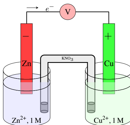
Figure ?? The Daniell galvanic cell
