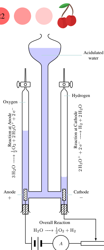
▲ Experimental set up for the electrolysis of water (Hoffman's voltameter). Oxygen is produced in the anode and hydrogen in the cathode.
