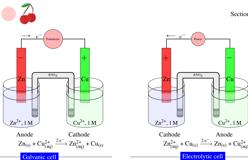
Figure 8.6 A galvanic cell produces voltage from a redox reaction, whereas an electrolytic cell uses voltage to produce a redox reaction. Anodes and cathodes have the opposite sign notation, electrons flow from anode to cathode, whereas ions move towards the electrode of same name (e.g anions migrate towards the anode). However, galvanic anodes are electrolytic cathodes and viceversa.
