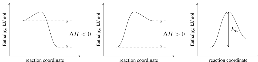
Figure ?? A set of reaction energy profiles displaying the energy of reaction and the activation energy: exothermic (left), endothermic (center), and endothermic (right)
