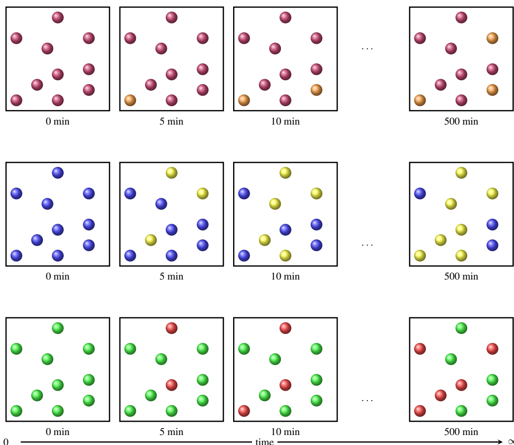
Figure 4.1 Three equilibrium situations. (Top Panel) At equilibrium, there are more reactants than products. (Central Panel) At equilibrium, there are more products than reactants. (Bottom Panel) At equilibrium, there are as many products as reactants.
