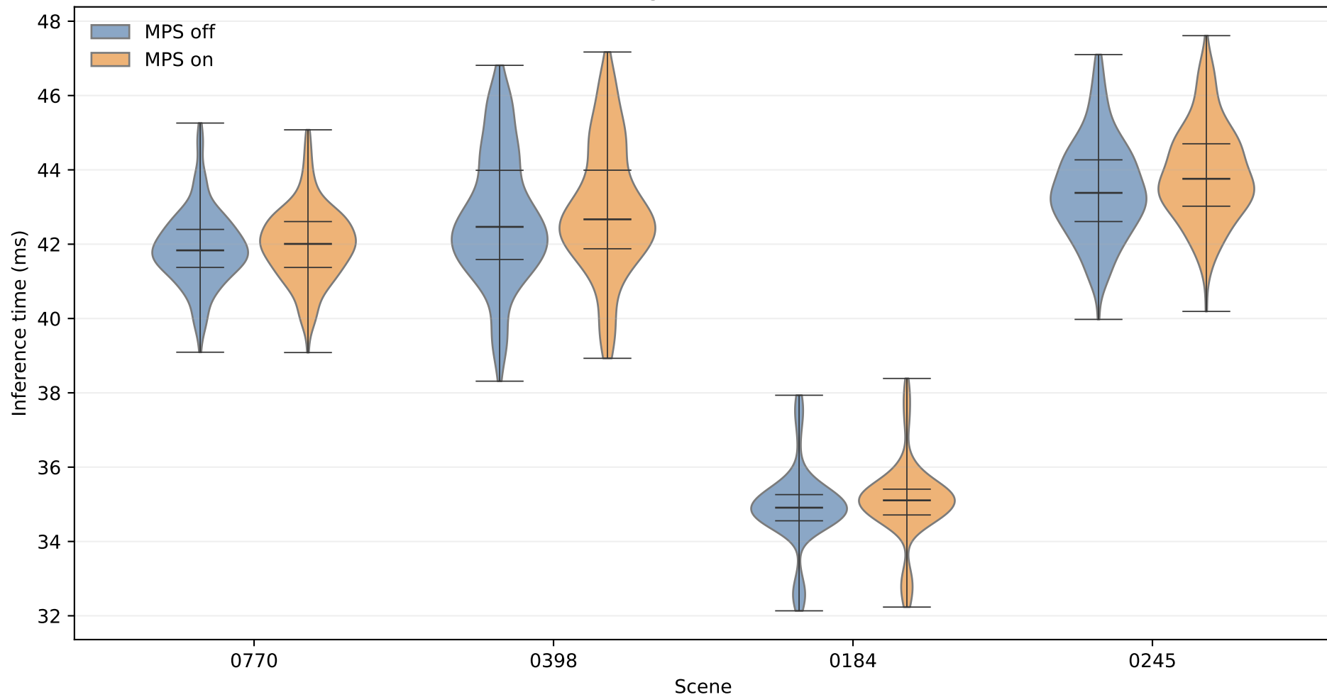
mask-rcnn — single-model baseline ( \leq P99 )
