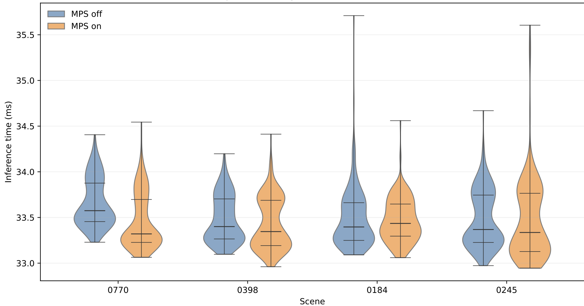
vit-upernet — single-model baseline ( \leq P99 )
