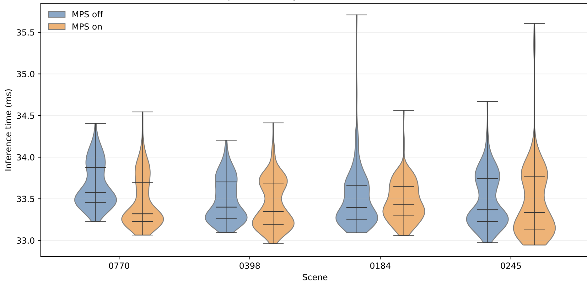
vit-upernet — single-model baseline ( \leq P99 )
