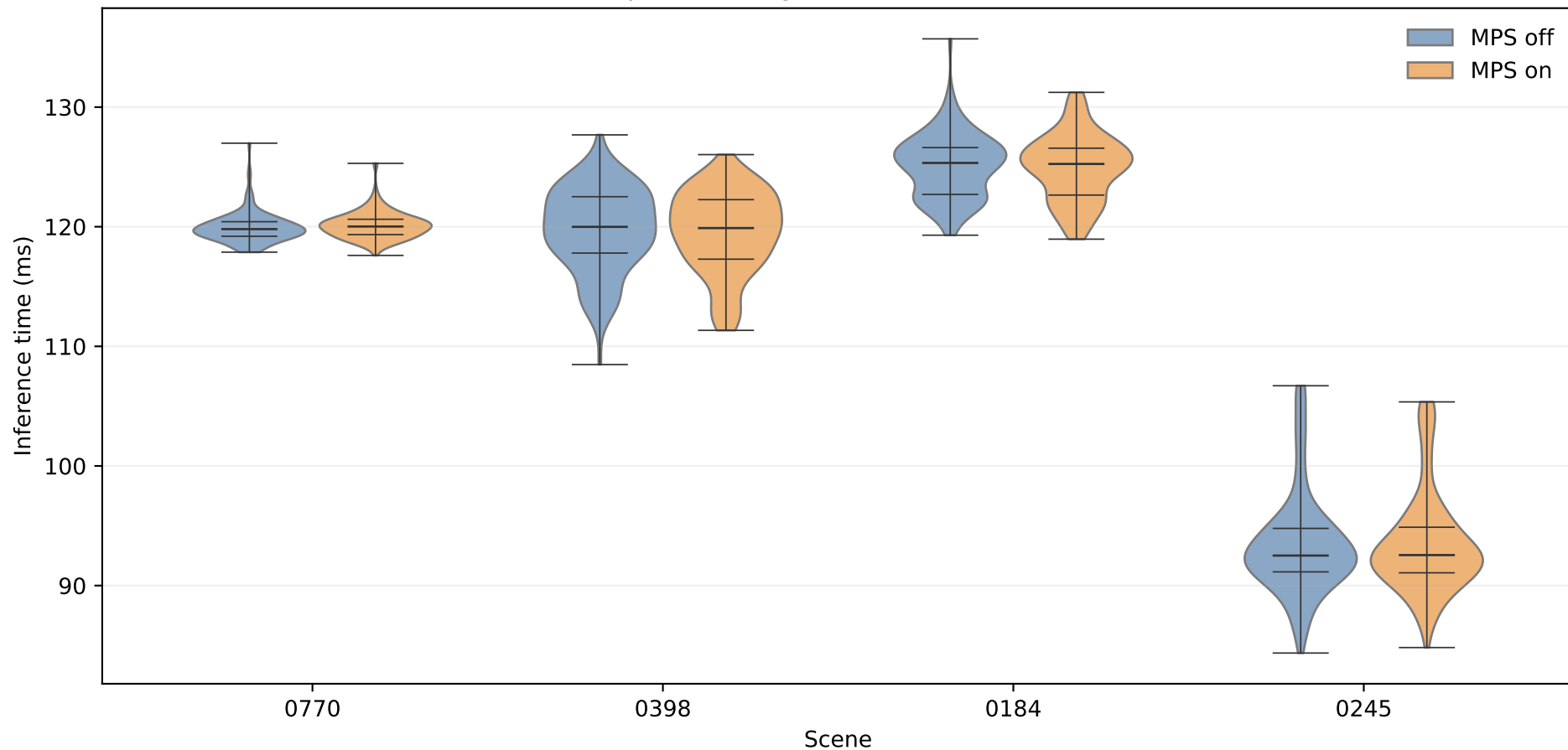
centerpoint — single-model baseline ( \leq P99 )
