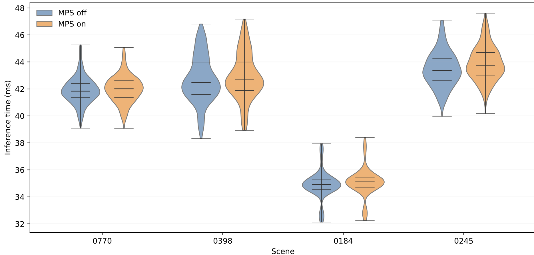
mask-rcnn — single-model baseline ( \leq P99 )
