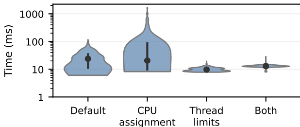
(c) ViT worker scheduling
