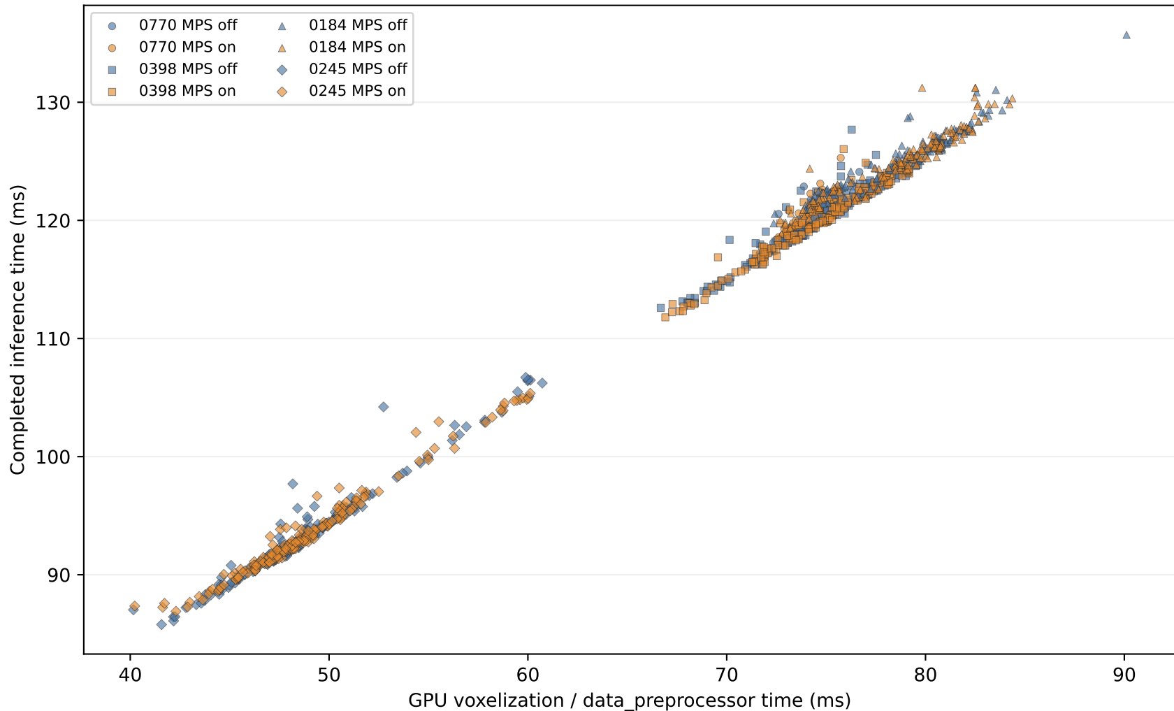
CenterPoint: voxelization tracks inference variation
