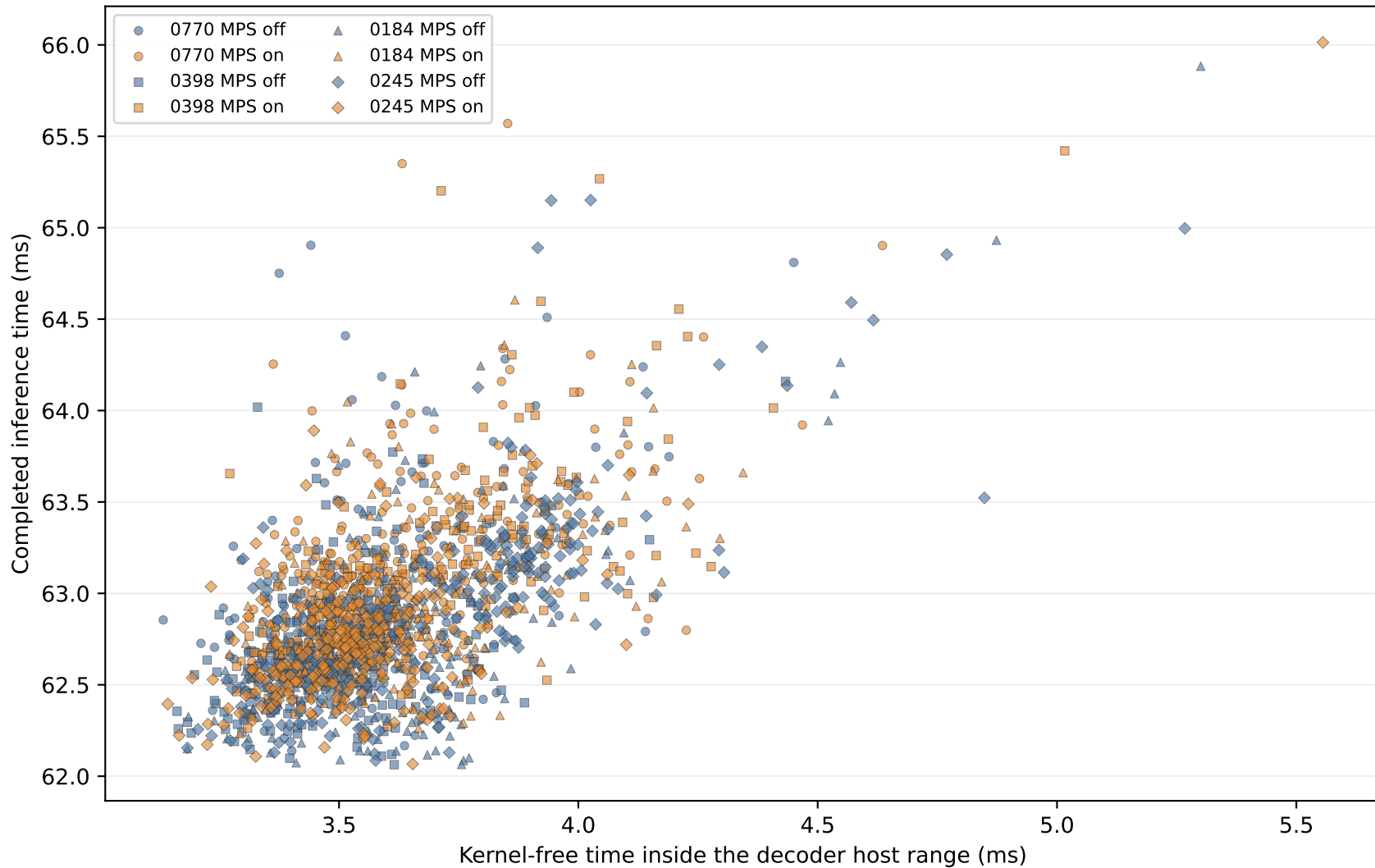
DINO: decoder host gaps — P1-P99 filtered
