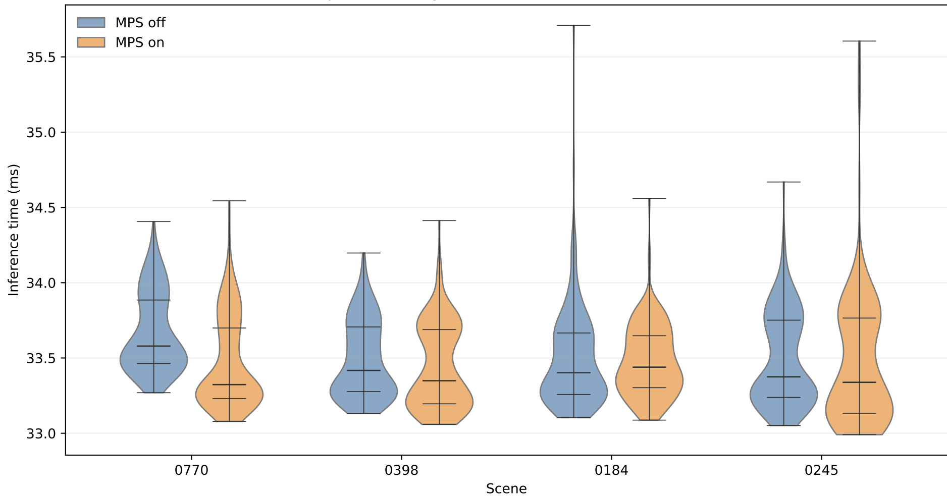
vit-upernet — single-model baseline (P1-P99 filtered)
