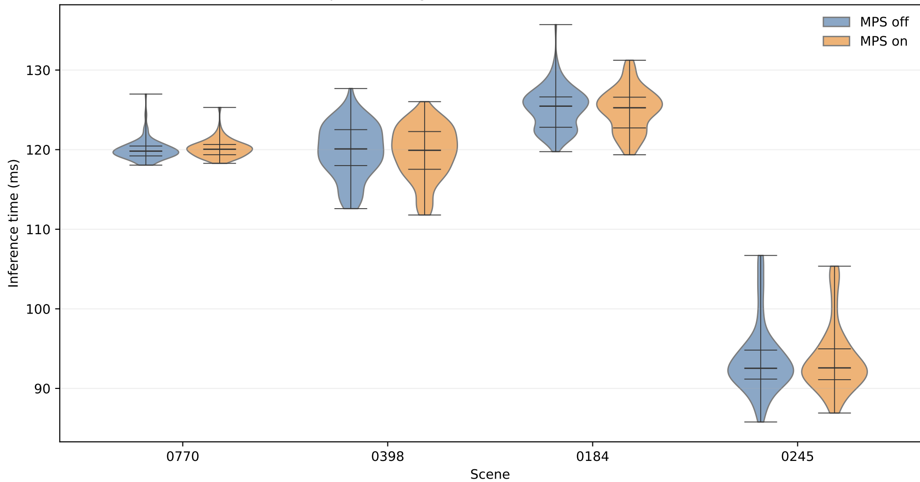
centerpoint — single-model baseline (P1-P99 filtered)
