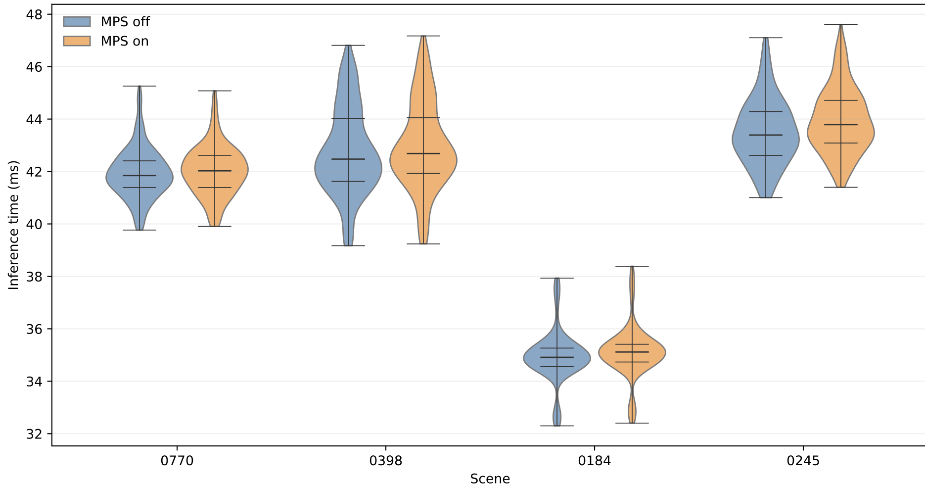
mask-rcnn — single-model baseline (P1-P99 filtered)
