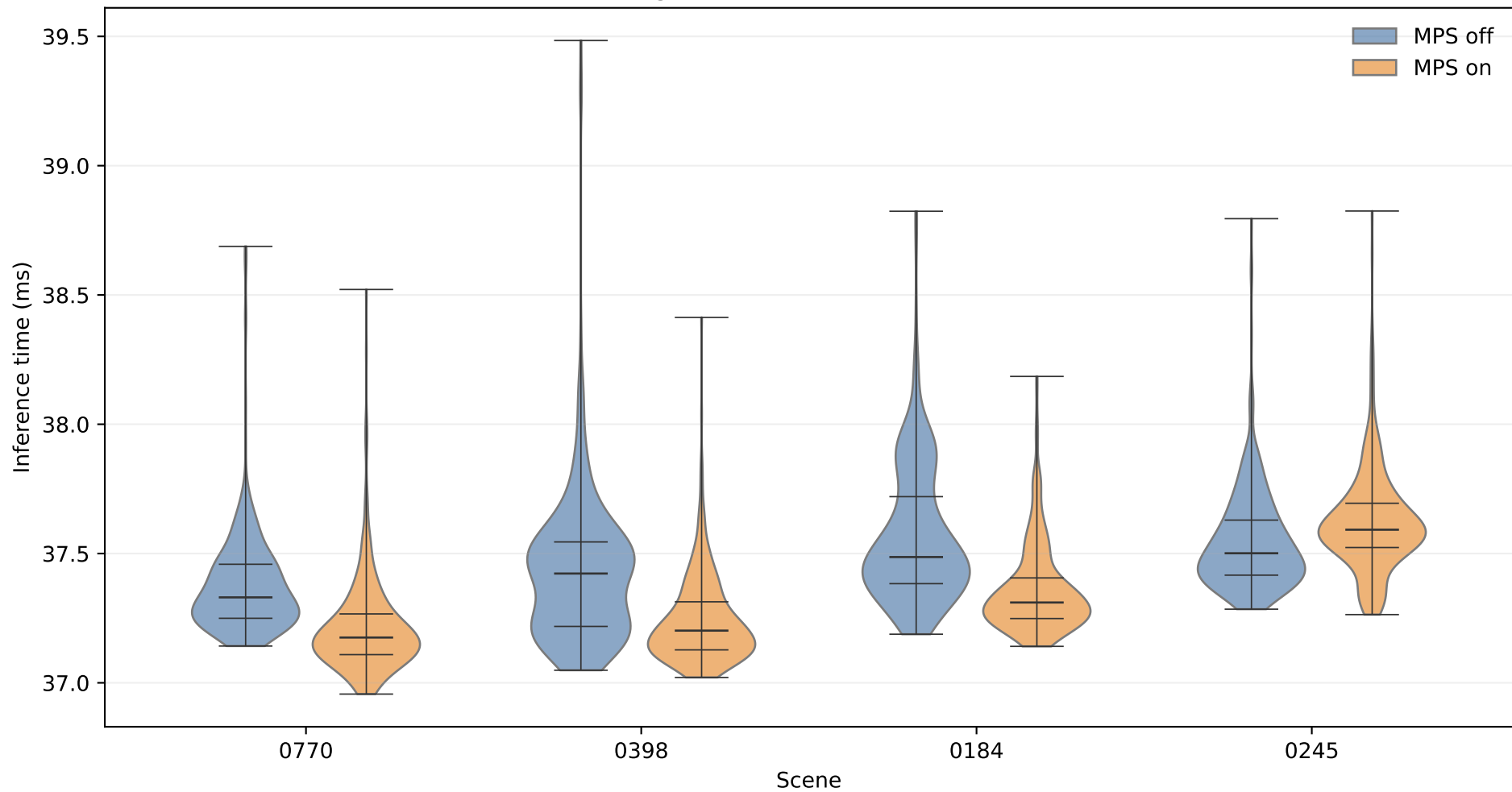
3dssd — single-model baseline (P1-P99 filtered)
