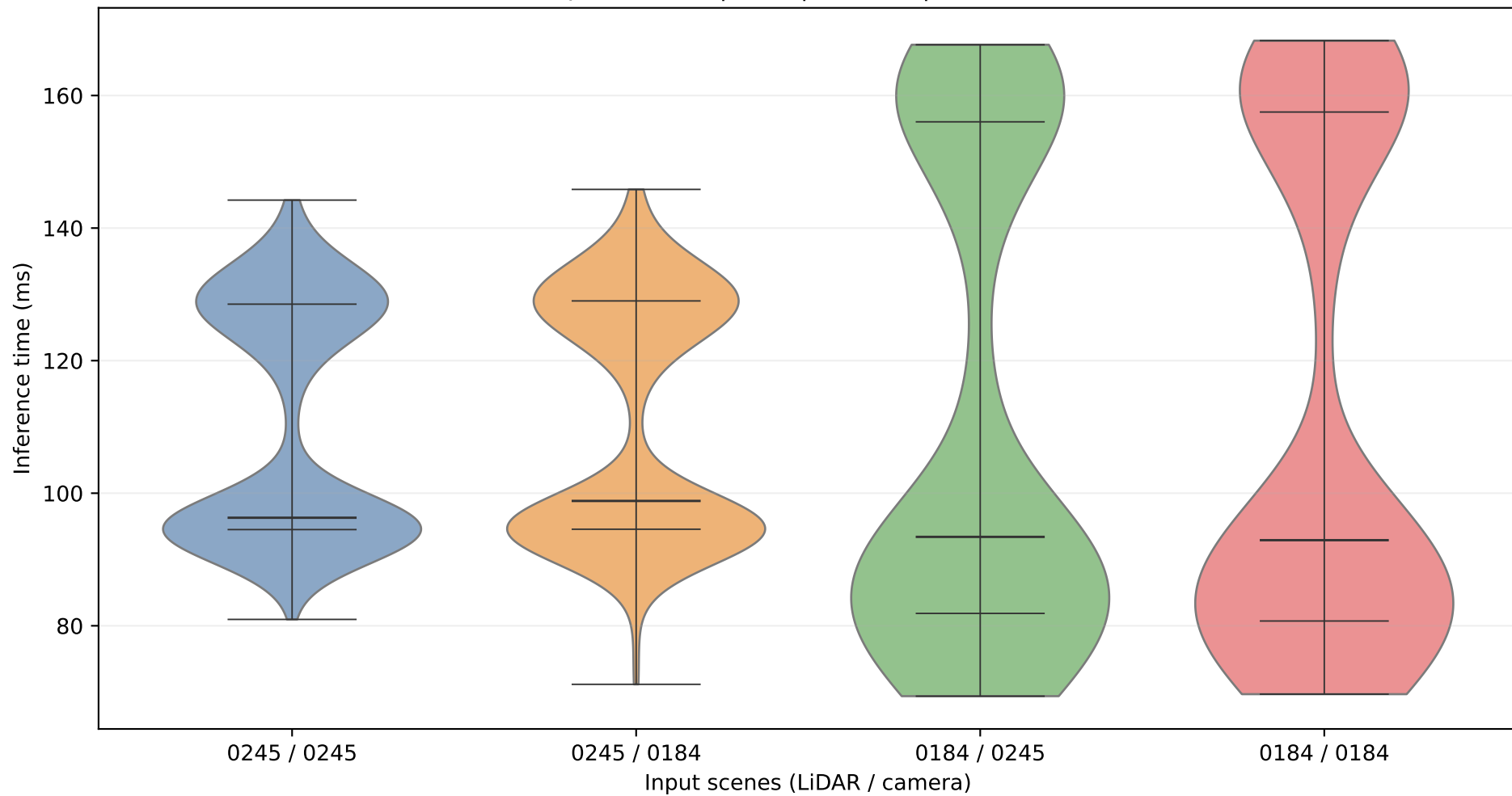
centerpoint+dino | dino | MPS off | P1-P99 filtered
