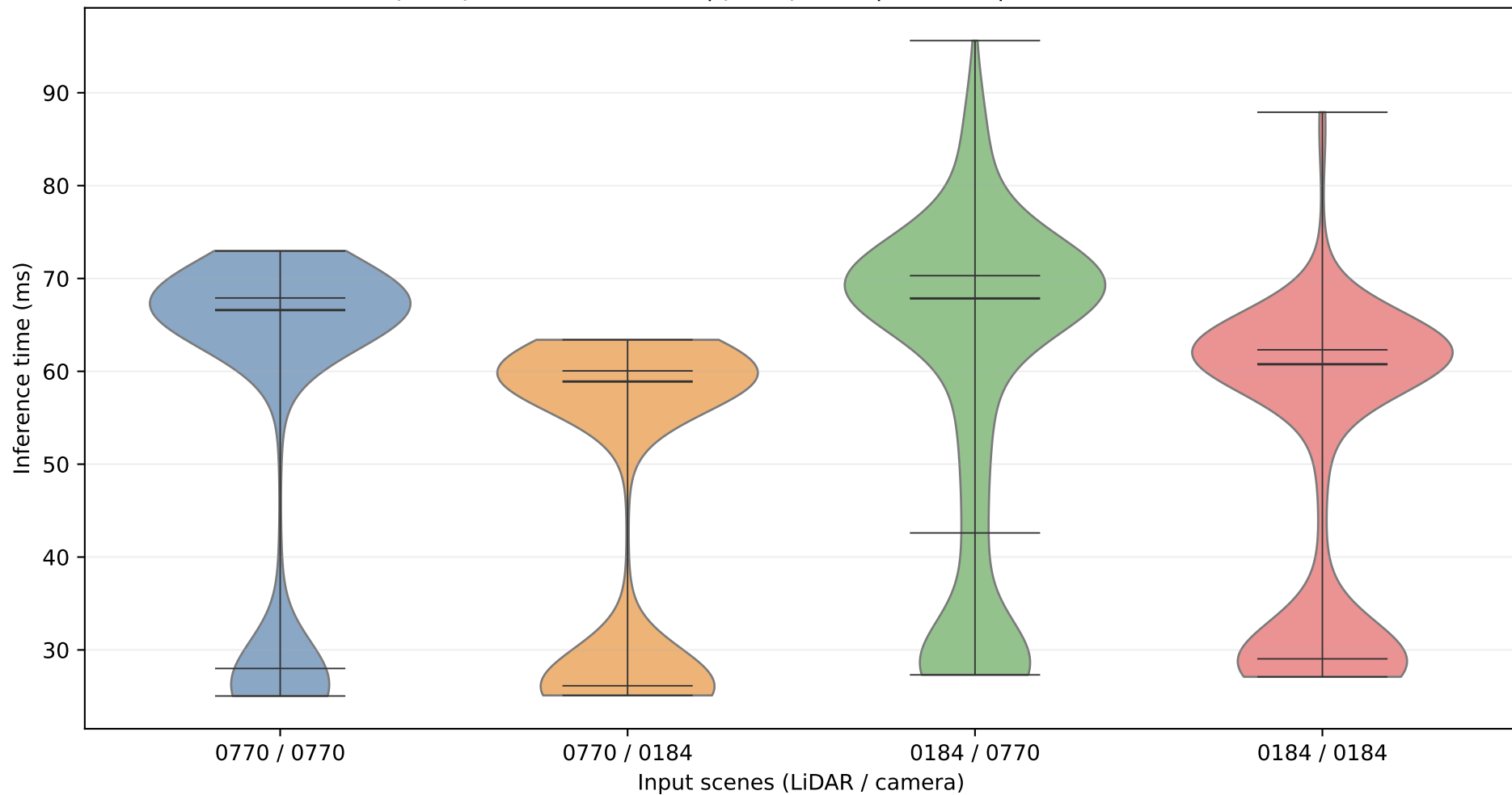
pointpillars+mask-rcnn | pointpillars | MPS off | P1-P99 filtered
