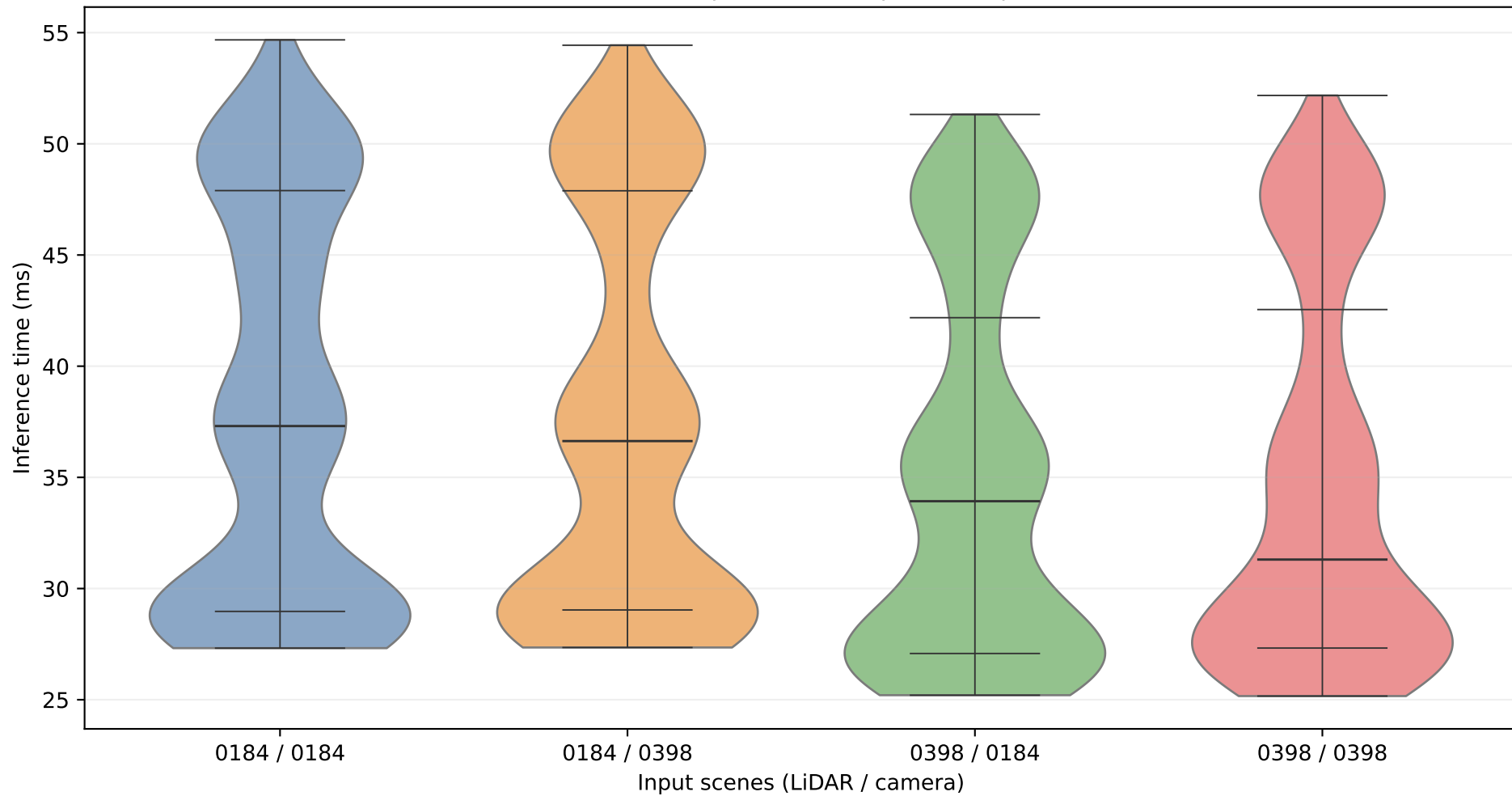
pointpillars+vit-upernet | pointpillars | MPS on | P1-P99 filtered
