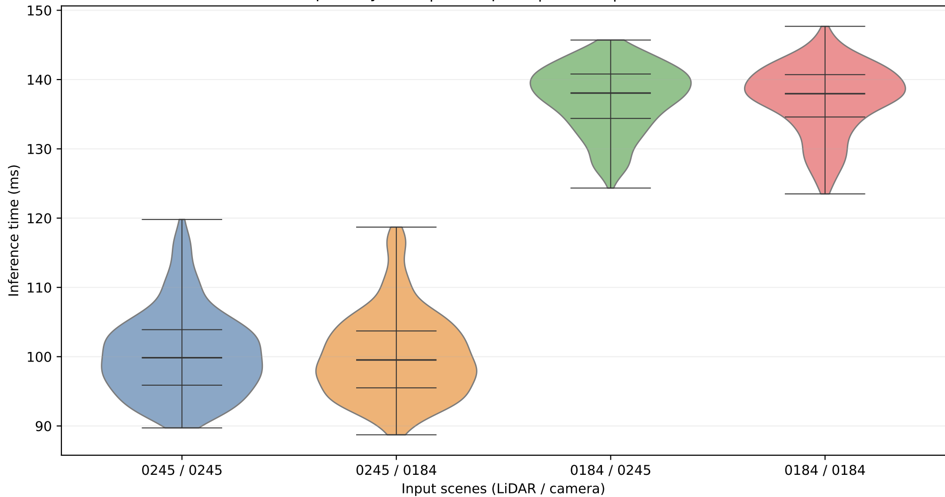
centerpoint+yolov3 | centerpoint | MPS on | P1-P99 filtered
