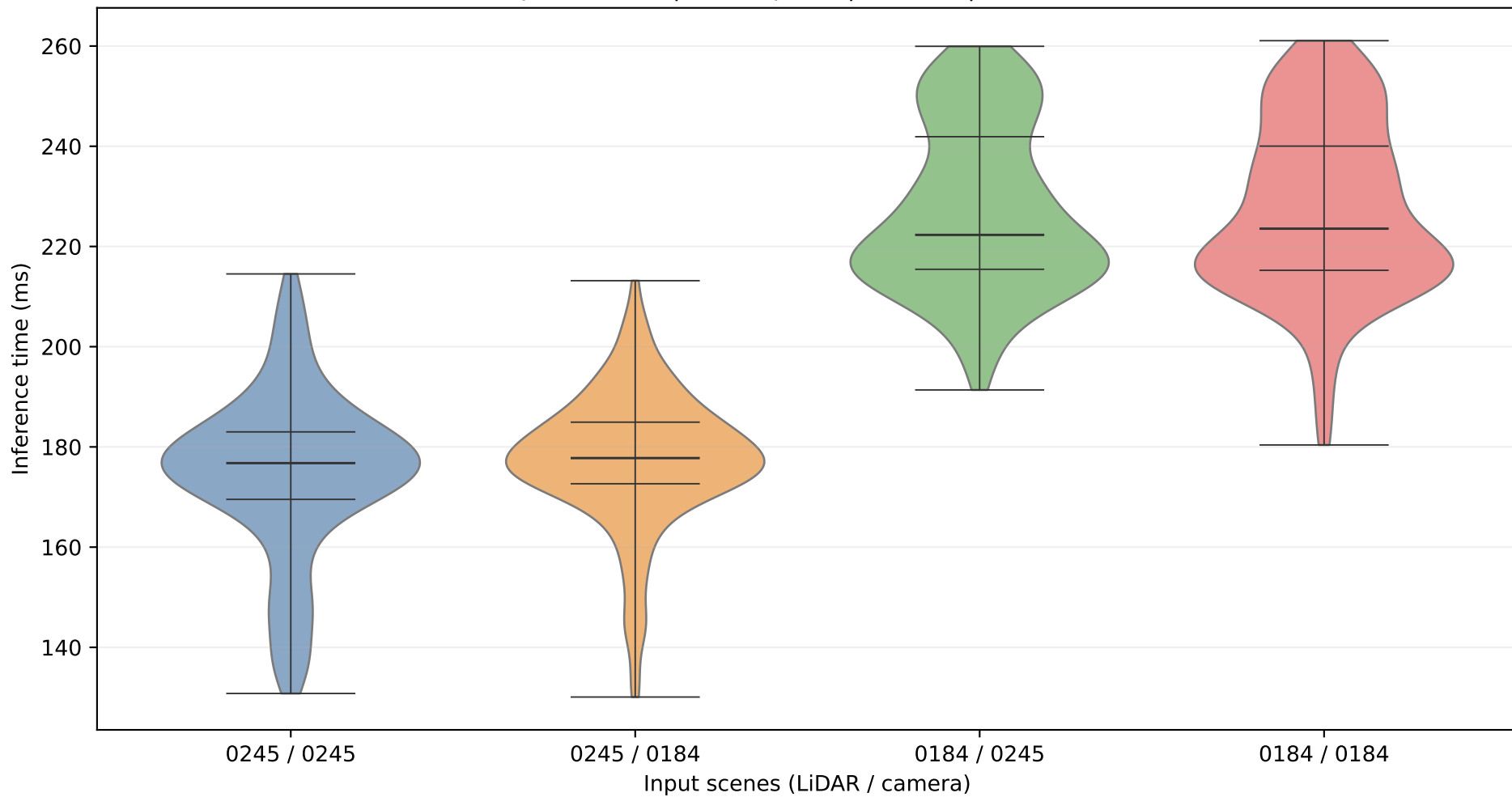
centerpoint+dino | centerpoint | MPS on | P1-P99 filtered
