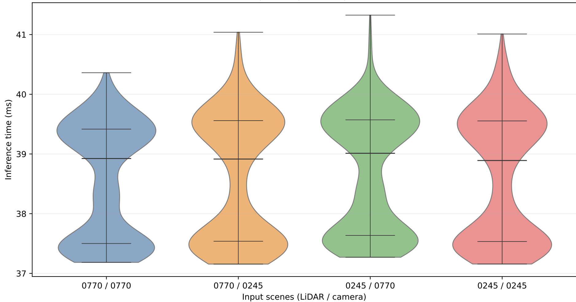
3dssd+yolov3 | 3dssd | MPS on | P1-P99 filtered
