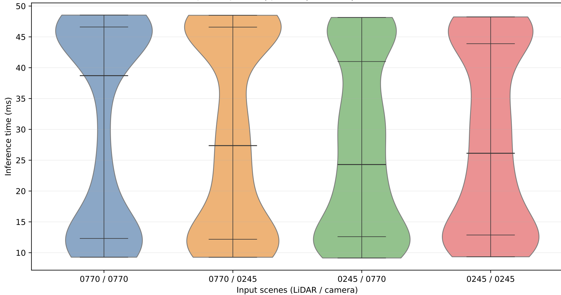
centerpoint+yolov3 | yolov3 | MPS off | P1-P99 filtered
