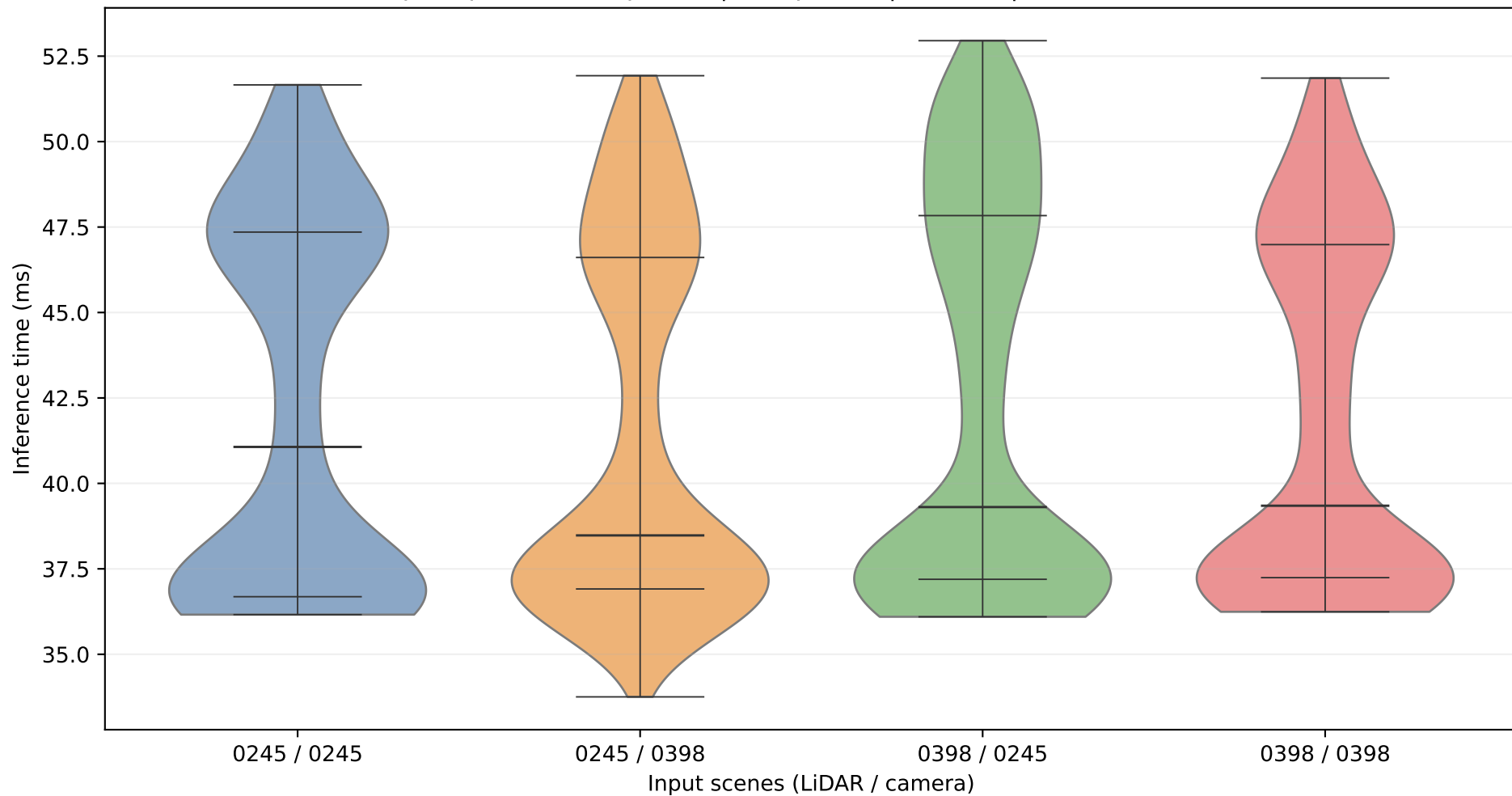
pointpillars+vit-upernet | vit-upernet | MPS off | P1-P99 filtered
