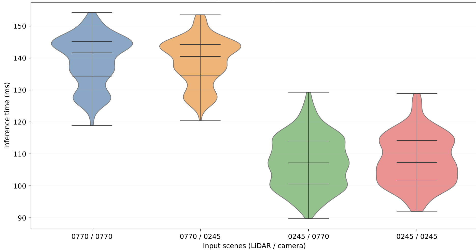
centerpoint+yolov3 | centerpoint | MPS off | P1-P99 filtered
