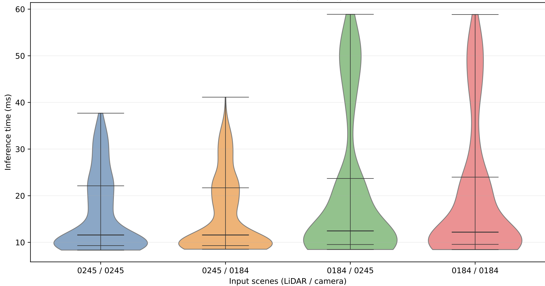
centerpoint+yolov3 | yolov3 | MPS on | P1-P99 filtered
