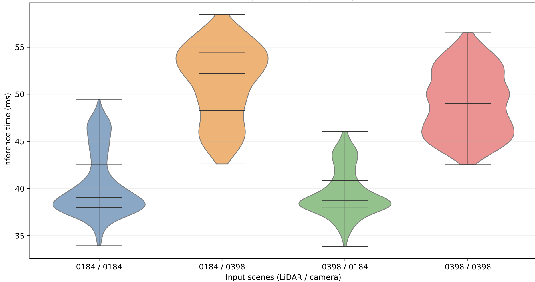
pointpillars+mask-rcnn | mask-rcnn | MPS on | P1-P99 filtered
