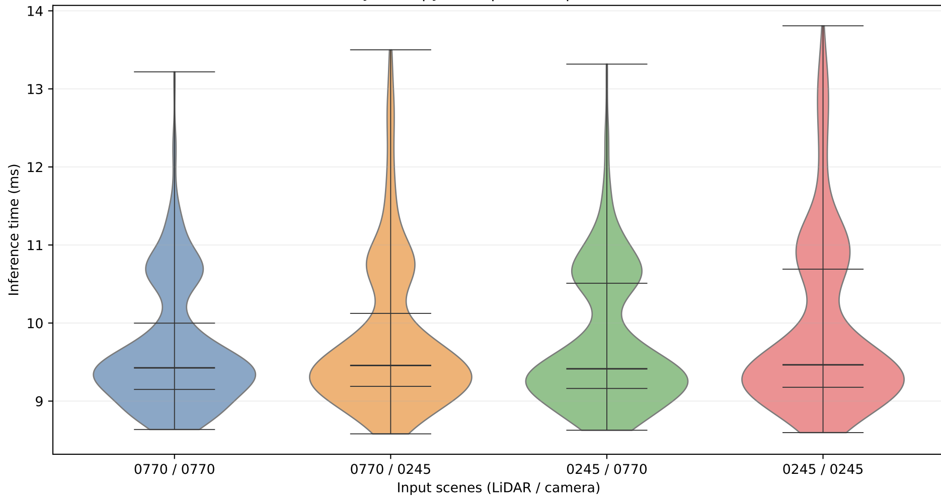
3dssd+yolov3 | yolov3 | MPS on | P1-P99 filtered
