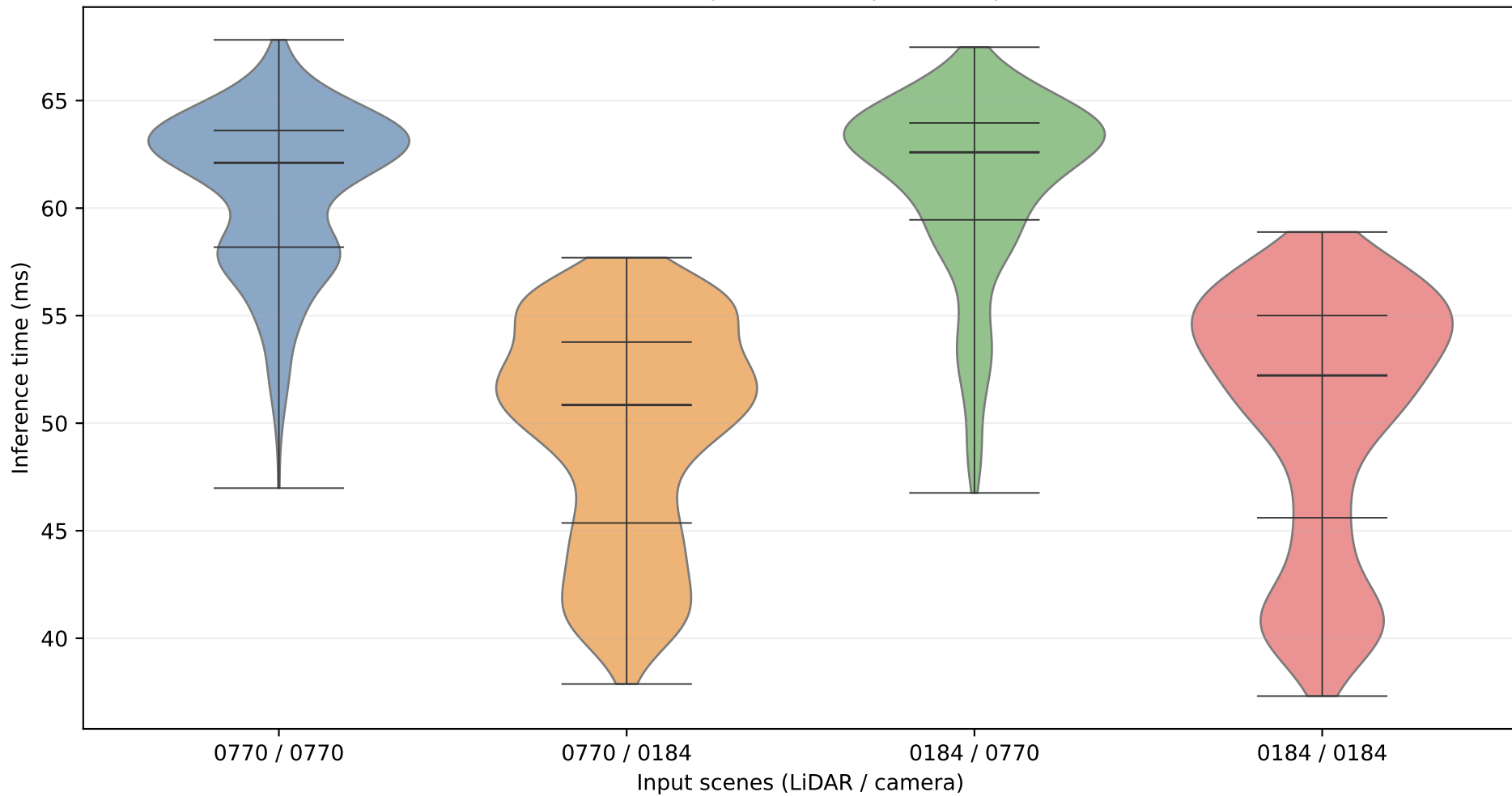
pointpillars+mask-rcnn | mask-rcnn | MPS off | P1-P99 filtered
