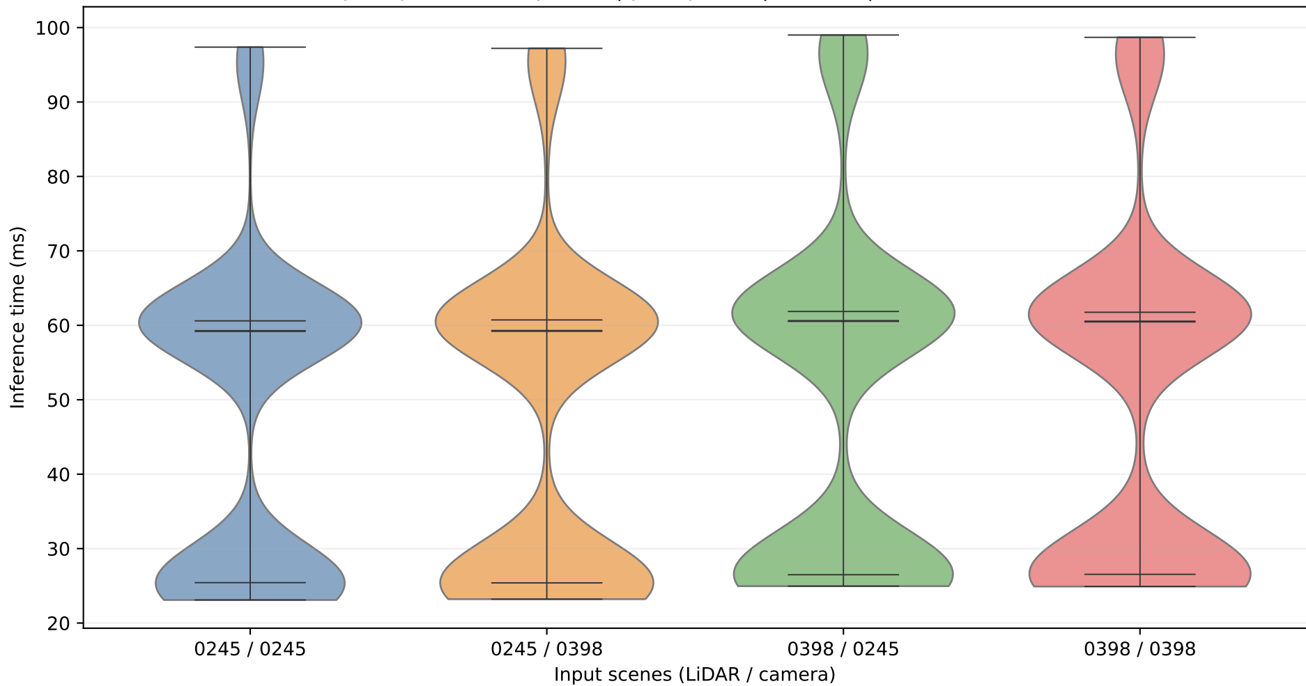
pointpillars+vit-upernet | pointpillars | MPS off | P1-P99 filtered
