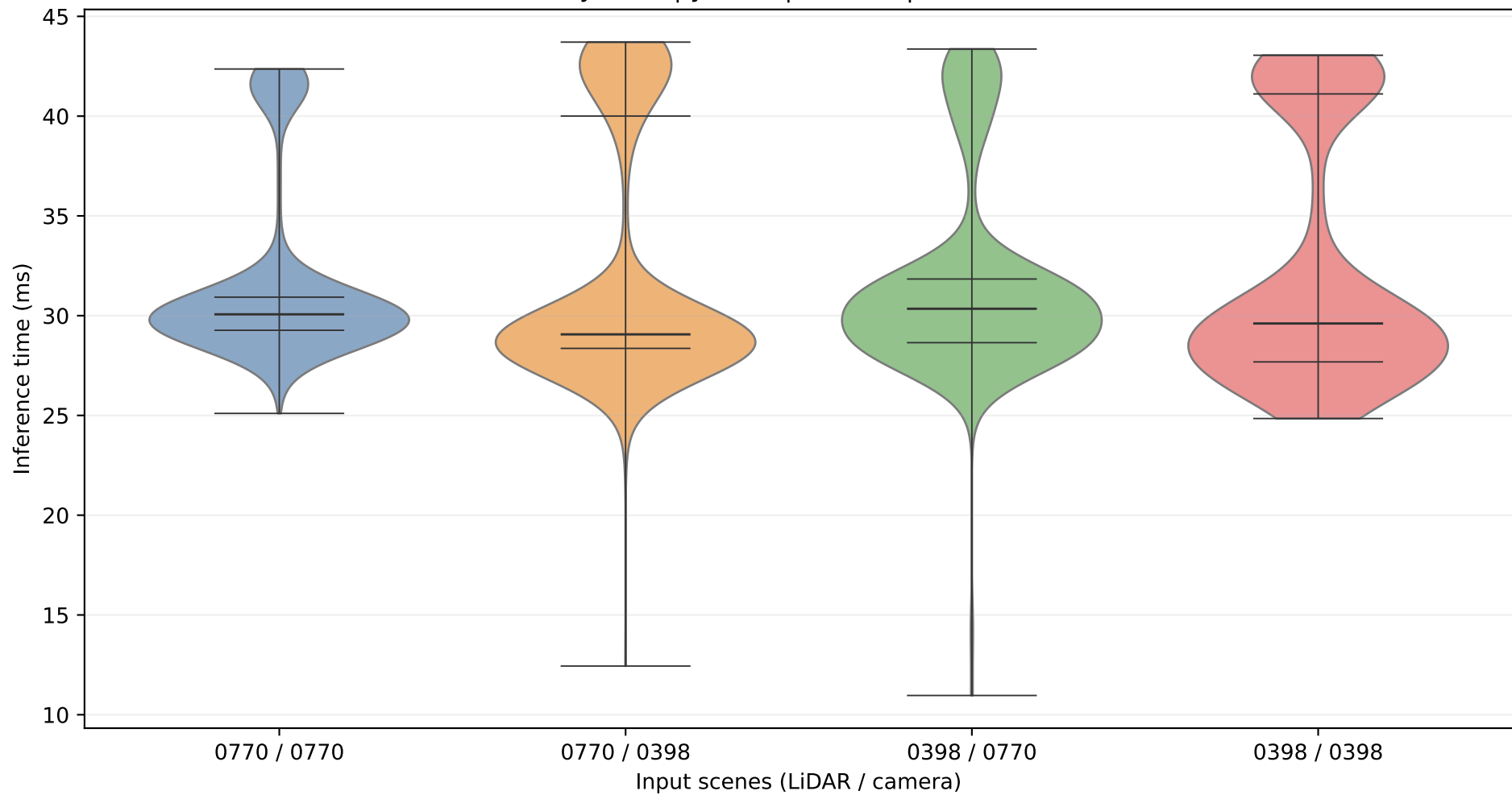
3dssd+yolov3 | yolov3 | MPS off | P1-P99 filtered
