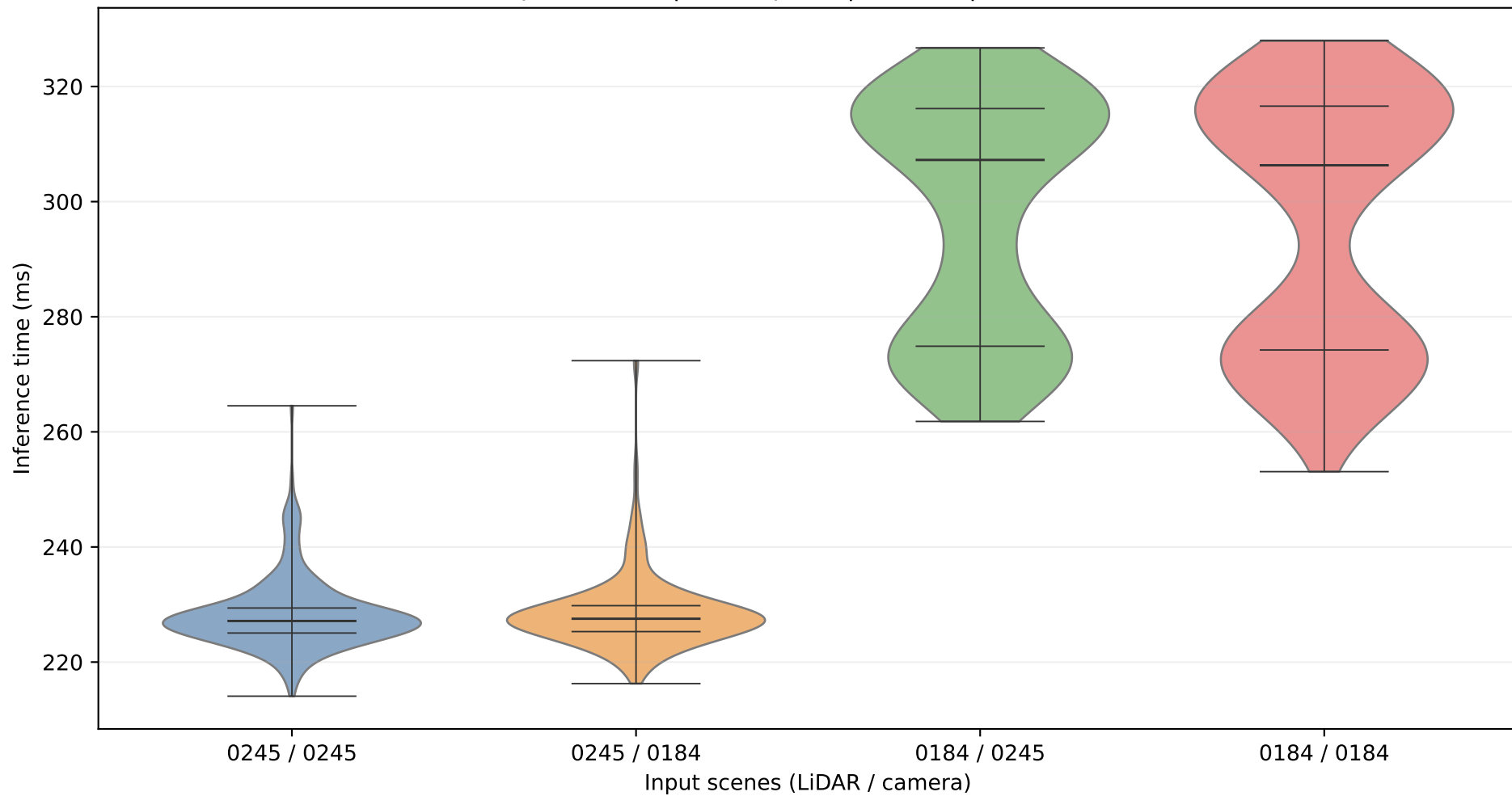
centerpoint+dino | centerpoint | MPS off | P1-P99 filtered
