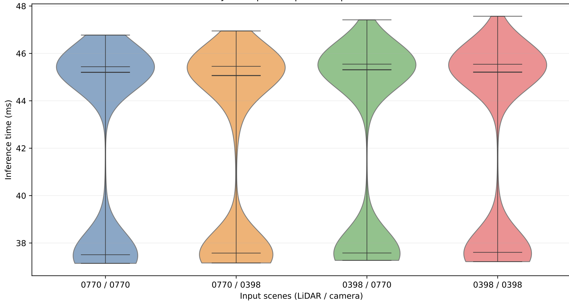
3dssd+yolov3 | 3dssd | MPS off | P1-P99 filtered
