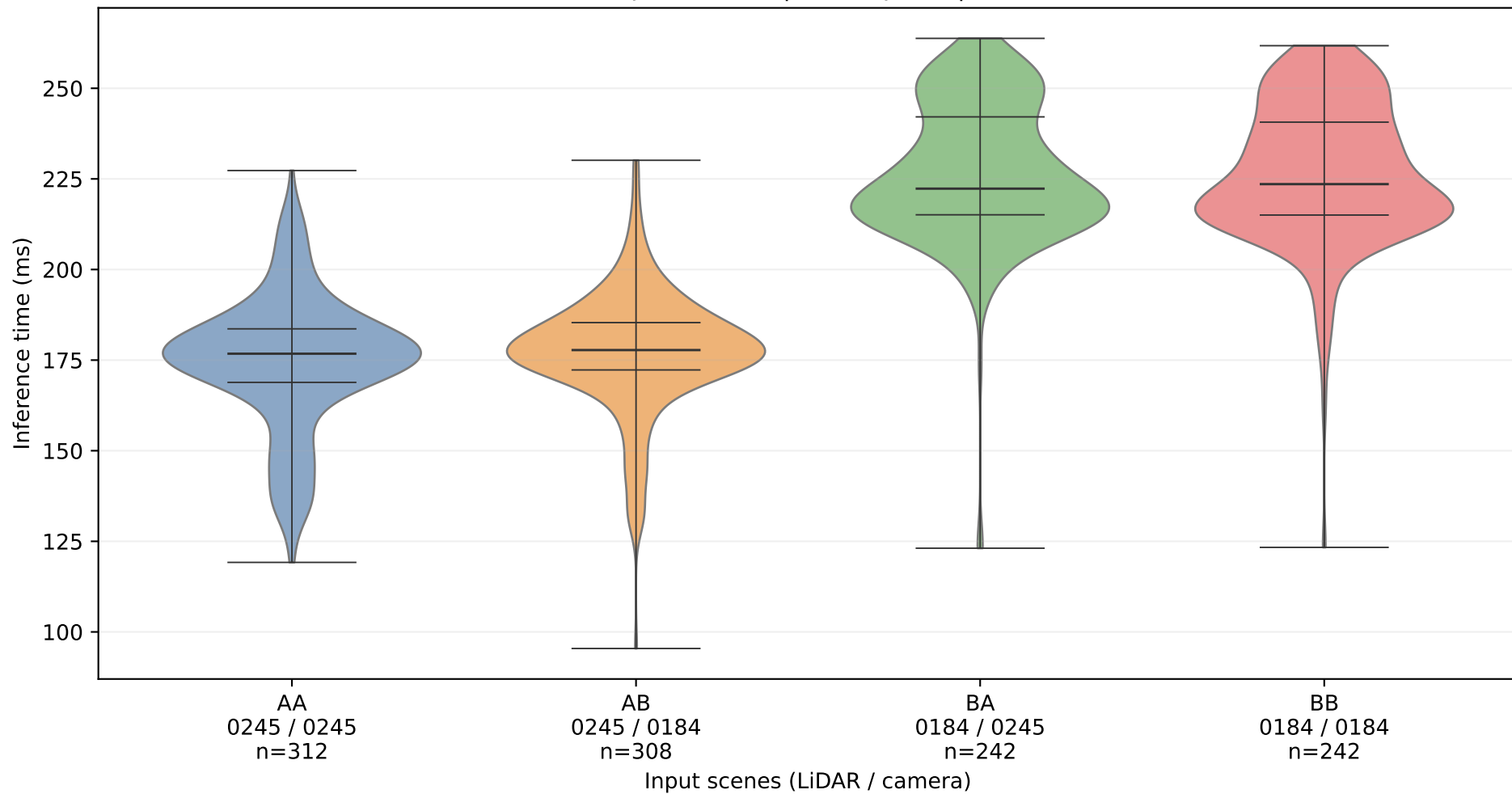
centerpoint+dino | centerpoint | MPS on
