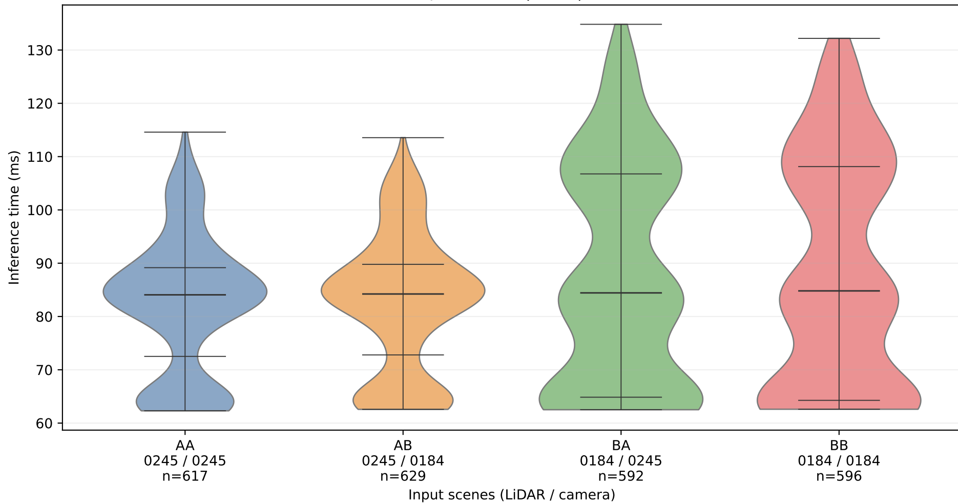
centerpoint+dino | dino | MPS on
