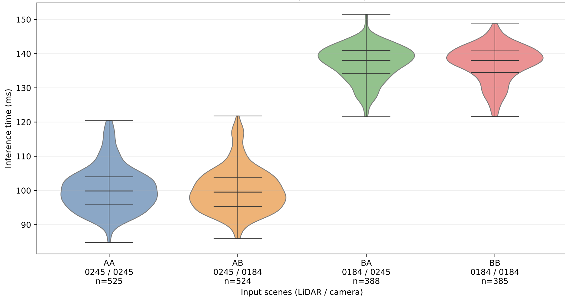
centerpoint+yolov3 | centerpoint | MPS on
