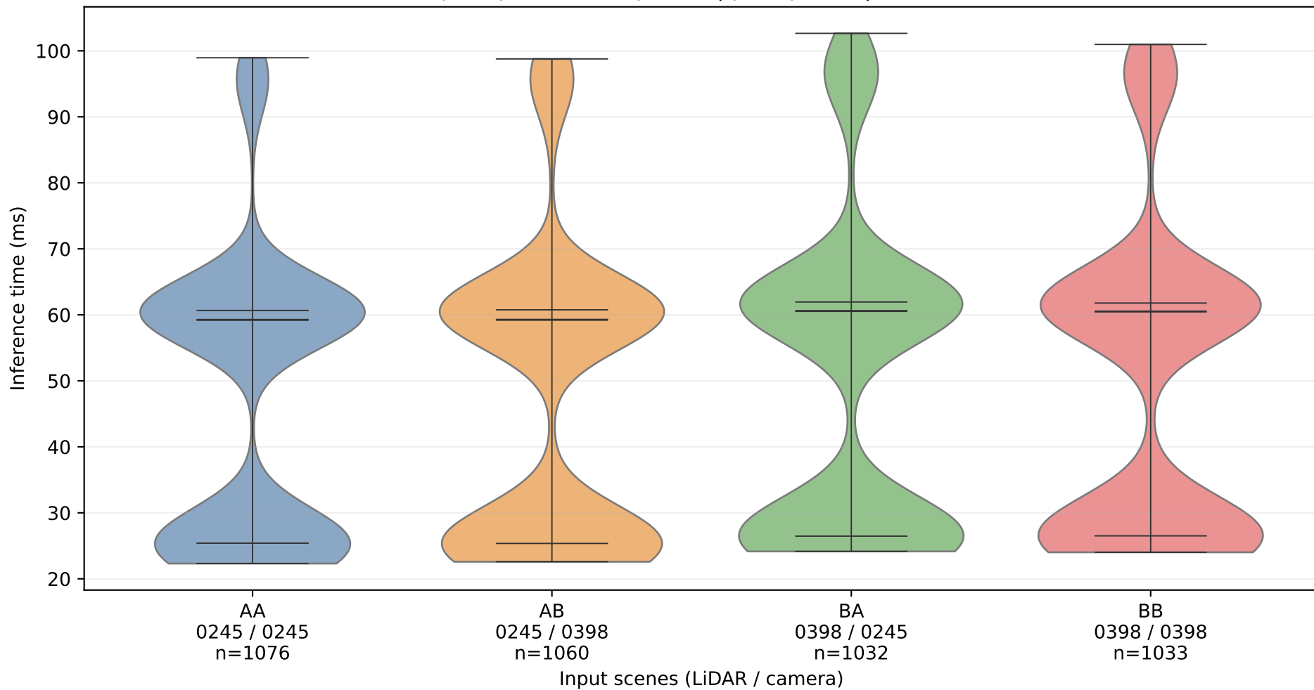
pointpillars+vit-upernet | pointpillars | MPS off
