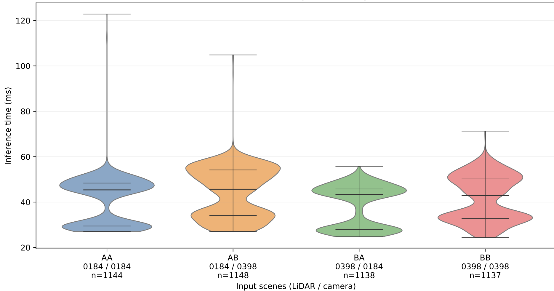
pointpillars+mask-rcnn | pointpillars | MPS on
