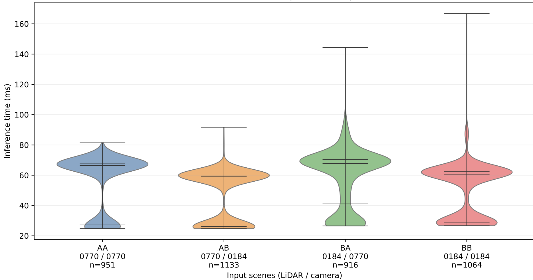
pointpillars+mask-rcnn | pointpillars | MPS off
