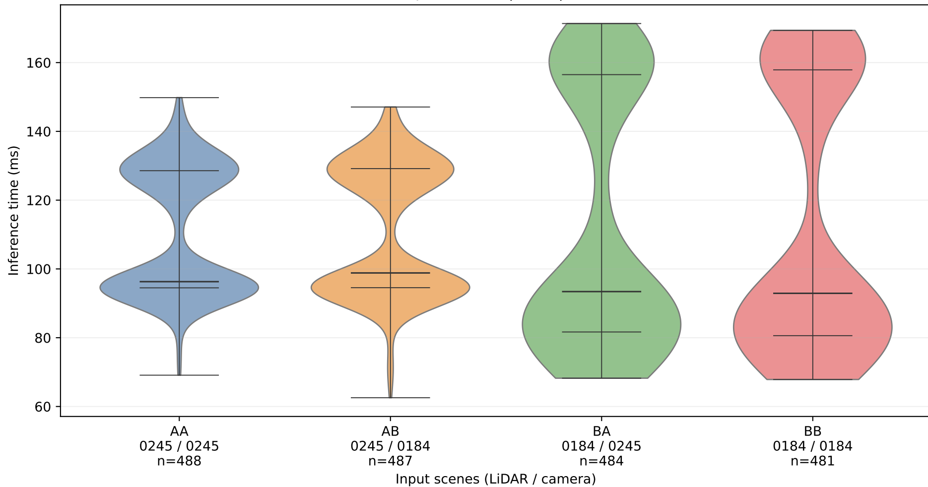
centerpoint+dino | dino | MPS off
