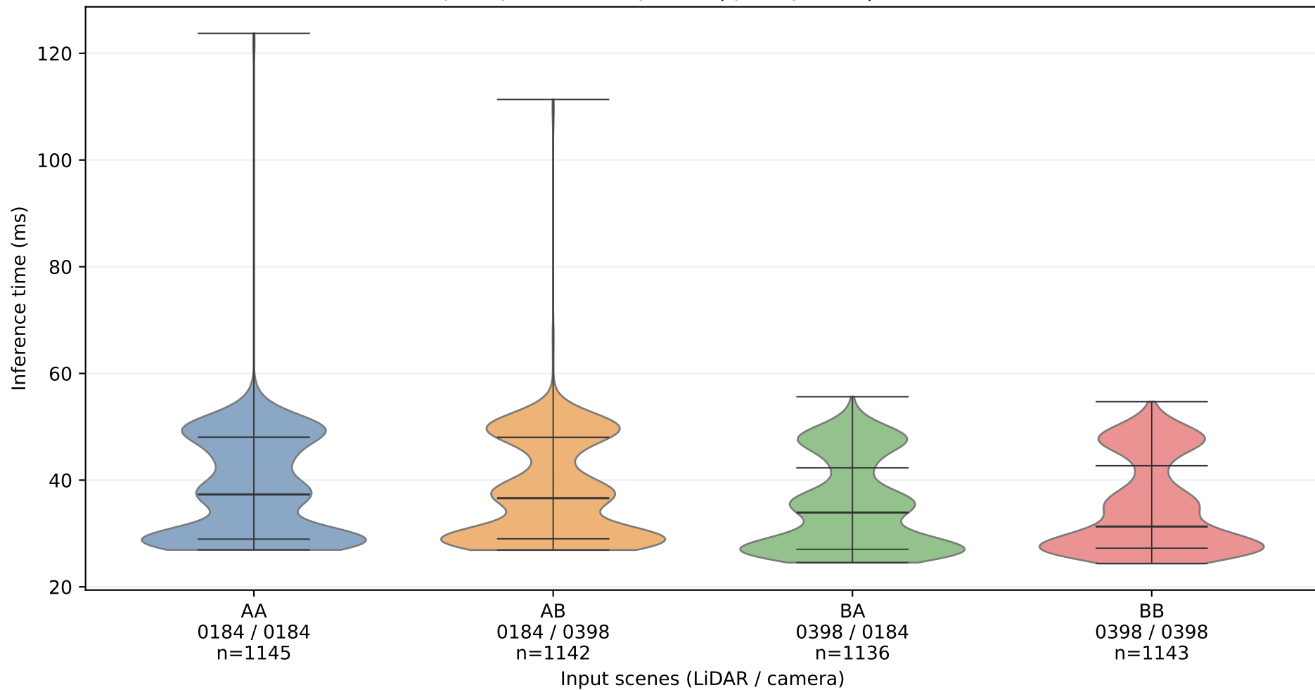
pointpillars+vit-upernet | pointpillars | MPS on
