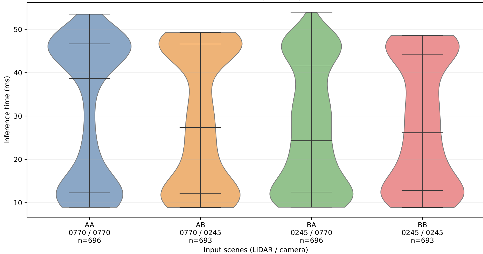
centerpoint+yolov3 | yolov3 | MPS off
