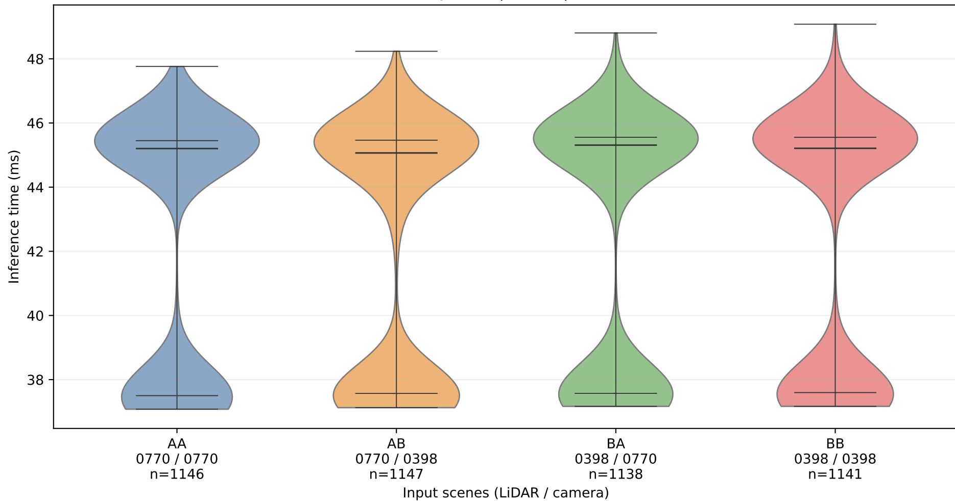
3dssd+yolov3 | 3dssd | MPS off
