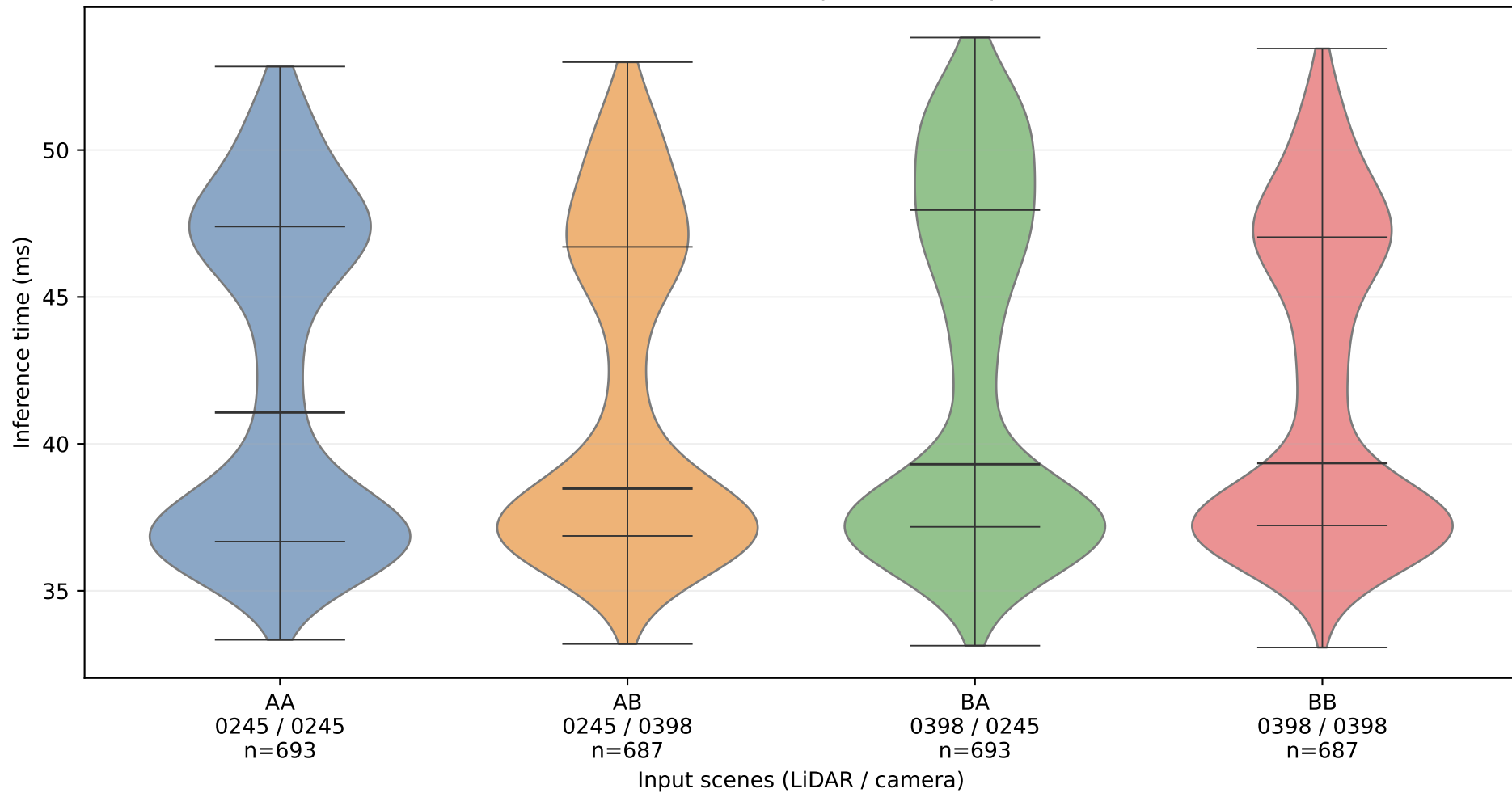
pointpillars+vit-upernet | vit-upernet | MPS off
