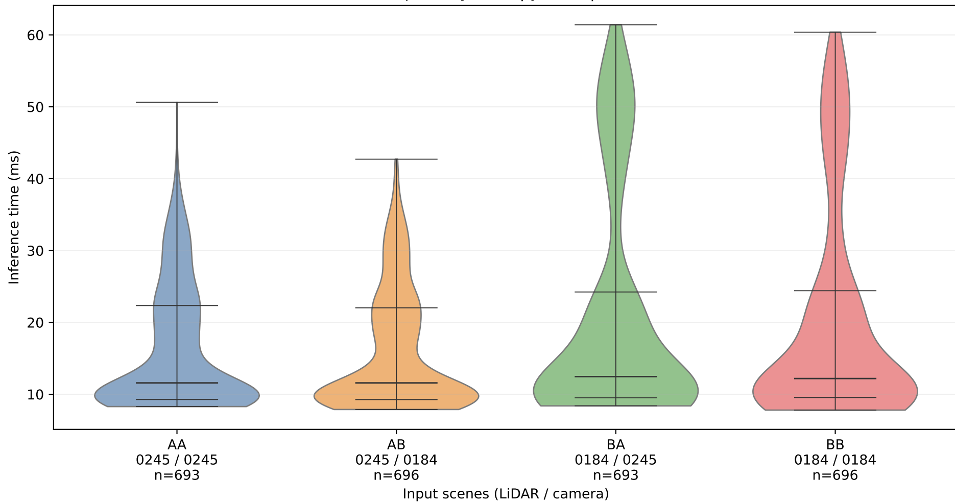
centerpoint+yolov3 | yolov3 | MPS on
