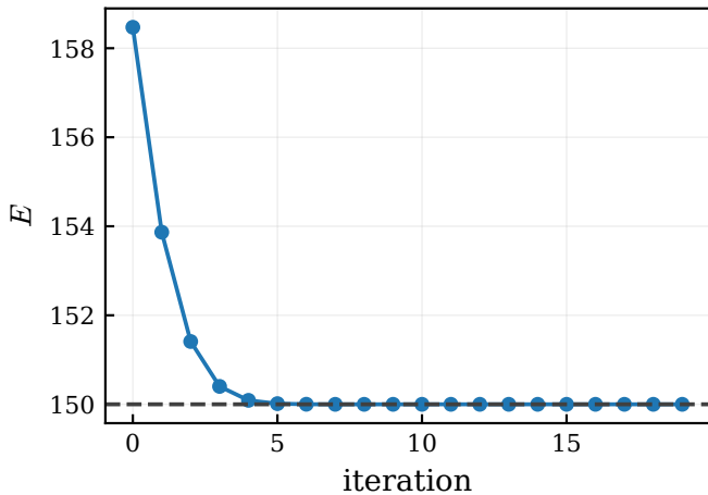
Figure 20: Energy during the \alpha optimization. The dashed line is the exact non-interacting energy E = 150 .
