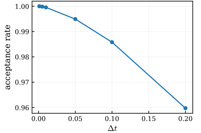
Figure 12: Importance-sampling acceptance rate in three dimensions at \alpha = 0.5 .
