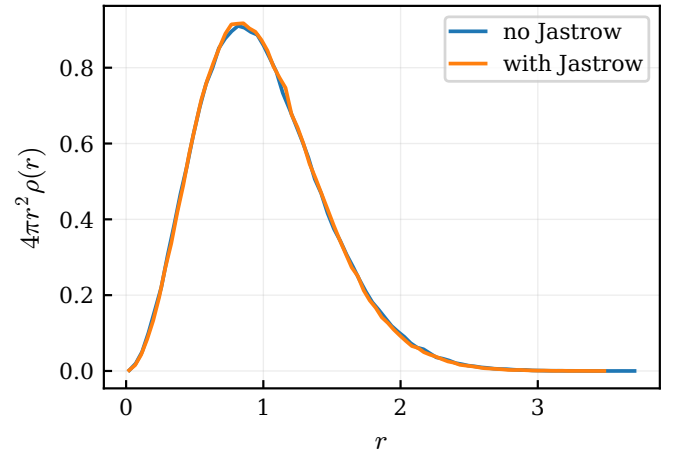
Figure 27: Radial probability distribution 4\pi r^2 \rho(r) with and without the Jastrow factor.
