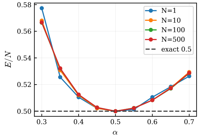
Figure 1: Brute-force Metropolis energy per particle in one dimension. The dashed line is the exact value E/N = 0.5 .
