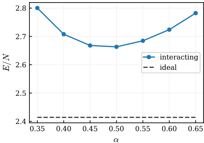
Figure 24: Interacting hard-core energy per particle for N = 50 particles.
