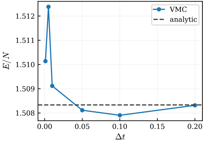
Figure 15: Importance-sampling energy in three dimensions at \alpha = 0.45 . The dashed line is the analytical variational value.
