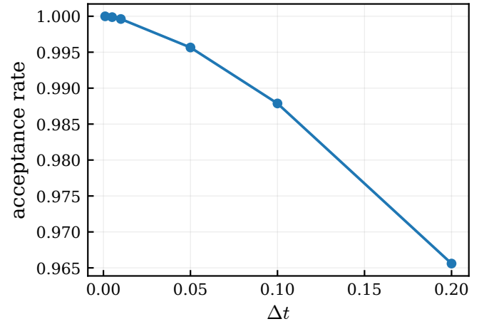
Figure 18: Importance-sampling acceptance rate in three dimensions at \alpha = 0.45 .
