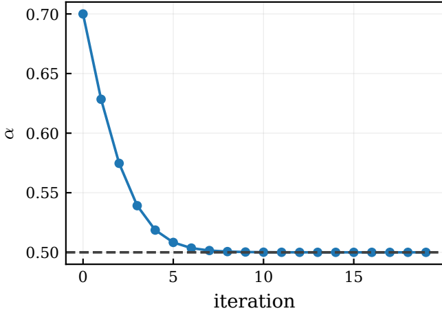
Figure 19: Optimization path for the variational parameter \alpha for N = 100 particles in three dimensions.
