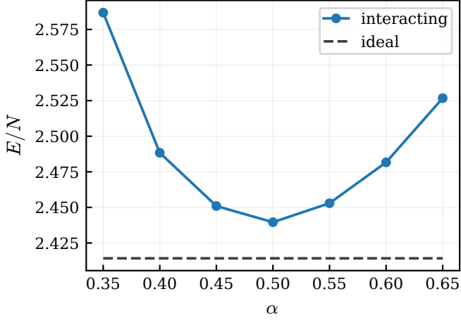
Figure 23: Interacting hard-core energy per particle for N = 10 particles.
