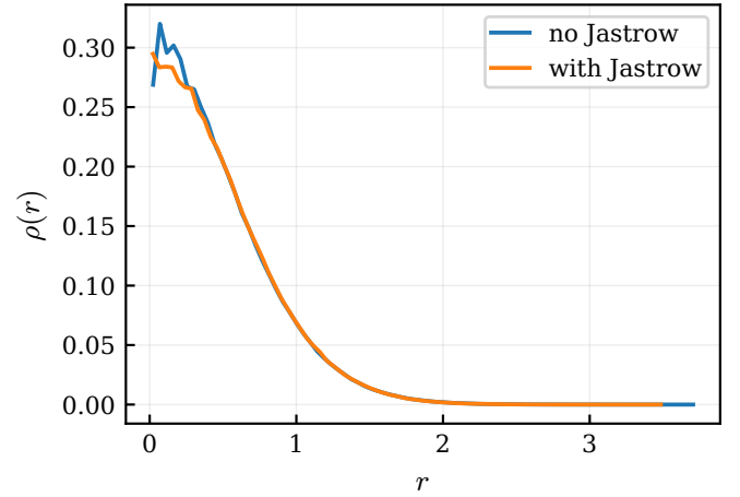
Figure 26: Radial one-body density with and without the Jastrow factor.
