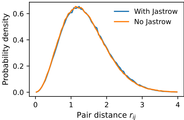
Pair-distance distribution
