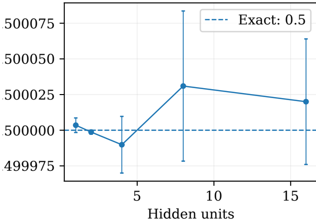
Figure 4: Hidden-node sweep for the non-interacting one-particle one-dimensional system. The plot uses a narrow vertical scale around E = 0.5 .
