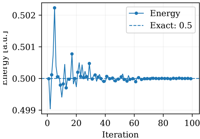
Figure 1: Brute-force Metropolis energy convergence for one particle in one dimension with two hidden nodes. The dashed line is the exact value E = 0.5 .
