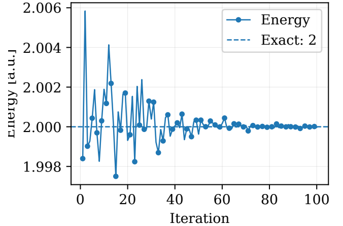
Figure 6: Importance-sampling energy convergence for two particles in two dimensions without interaction. The exact value is E = 2.0 .
