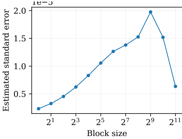
Figure 7: Blocking analysis for the one-dimensional importance-sampling run. The conservative error is taken from the maximum stable block-error estimate.
