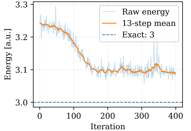
Figure 9: Longer interacting run with N_h = 16 . The energy decreases from about 3.23 to about 3.08, approaching but not reaching the exact value E = 3.0 .
