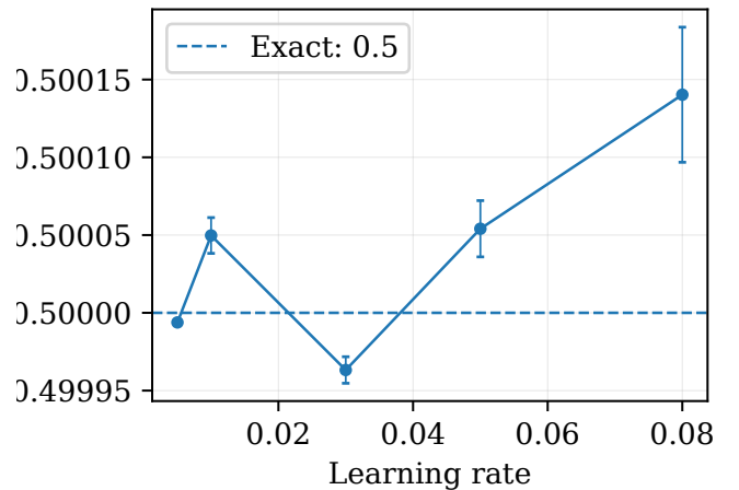
Figure 3: Learning-rate sweep for the non-interacting one-particle one-dimensional system. The scale is very narrow because all points are close to the exact energy.
