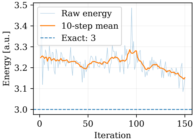
Figure 8: Initial interacting run for two particles in two dimensions. The result remains above the exact value E = 3.0 and shows significant fluctuations.
