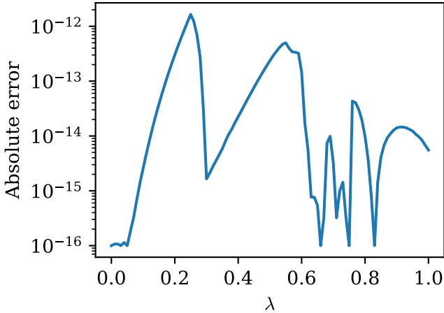
Figure 3: Absolute error of the one-qubit VQE ground-state energy relative to exact diagonalization. The error is dominated by numerical precision.
