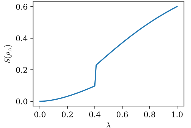
Figure 5: Von Neumann entropy of one qubit in the exact two-qubit ground state. The entropy grows with interaction strength and jumps when the ground-state sector changes.
