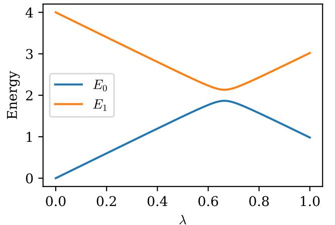
Figure 1: Exact eigenvalues of the two-level Hamiltonian as functions of \lambda . The coupling between basis states opens an avoided crossing near \lambda = 2/3 .
