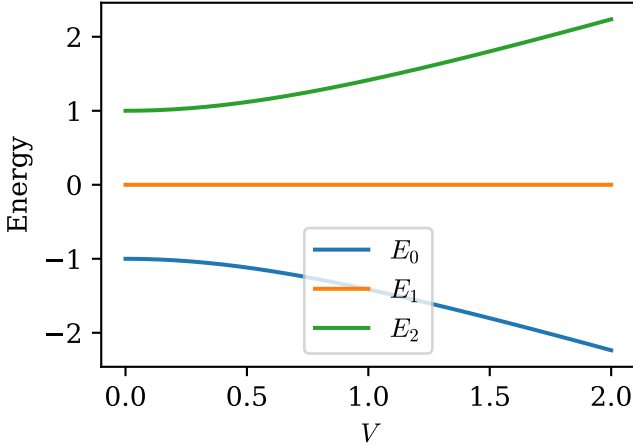
Figure 7: Exact Lipkin spectrum for J = 1 , \epsilon = 1 , and W = 0 . The spectrum consists of E = 0 and the branches E = \pm\sqrt{1 + V^2} .
