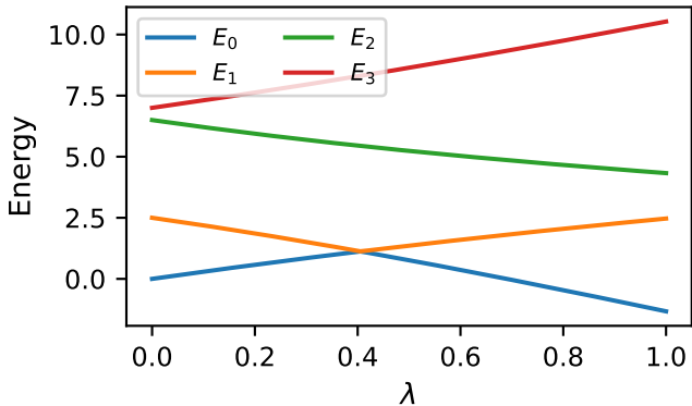
Two-qubit spectrum
