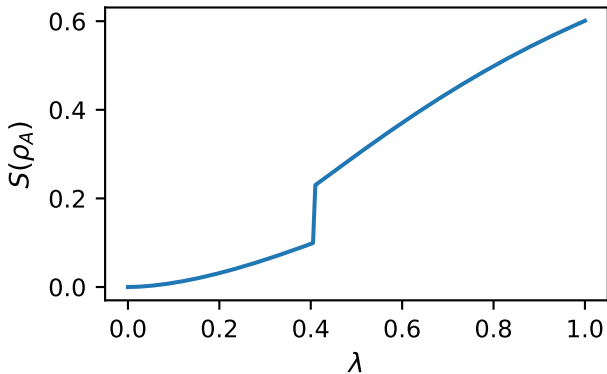
Ground-state entropy
