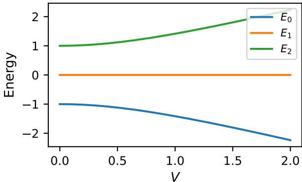
Lipkin spectrum, J = 1
