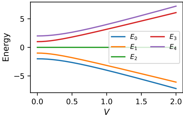
Lipkin spectrum, J = 2
