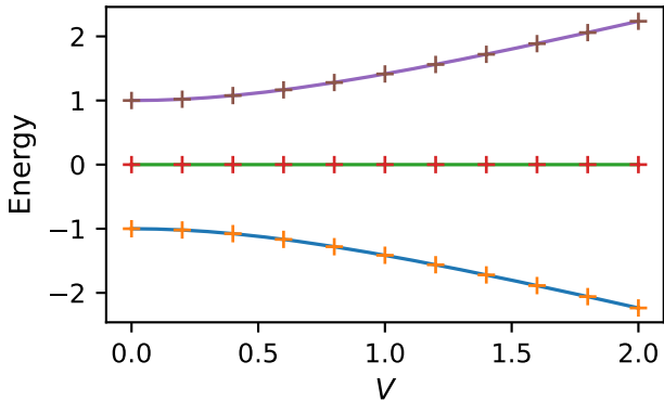
Excited-state VQE, J = 1
