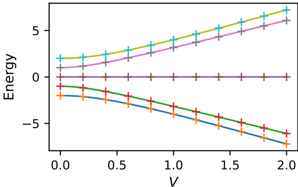
Excited-state VQE, J = 2
