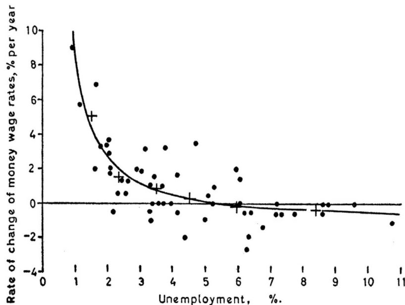
Figure 1: A. W. Phillips curve
