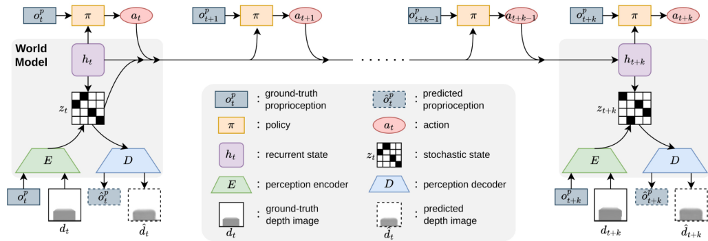
Figure 3.3.2: The WMP framework: the RSSM world model runs every k steps and its recurrent state feeds the policy [3]
