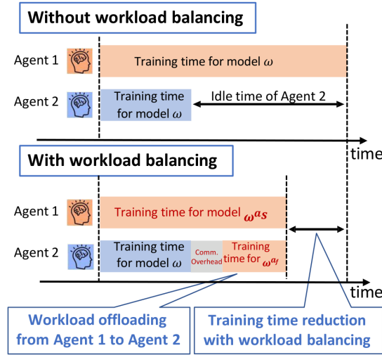
Figure 3.4.1: Training with and without workload balancing: offloading part of Agent 1's model to Agent 2 fills Agent 2's idle time and shortens the round [4]
