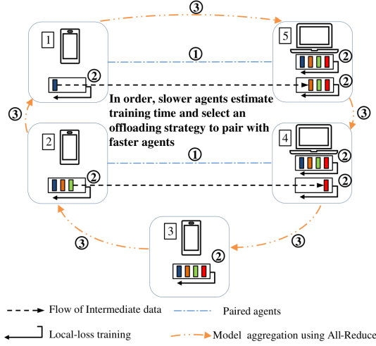
Figure 3.4.2: ComDML training round: agents 1 and 2 offload work to faster agents 5 and 4, agent 3 trains independently, and all models are aggregated with AllReduce [4]
