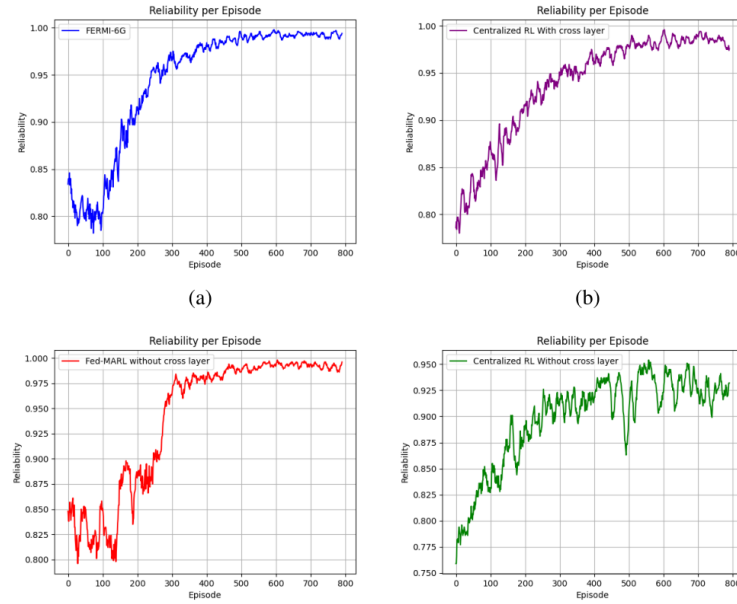
Figure 3.2.2: Reliability per episode: (a) FERMI-6G, (b) centralised RL with cross-layer optimisation, (c) Fed-MARL without cross-layer optimisation, (d) centralised RL [2]
