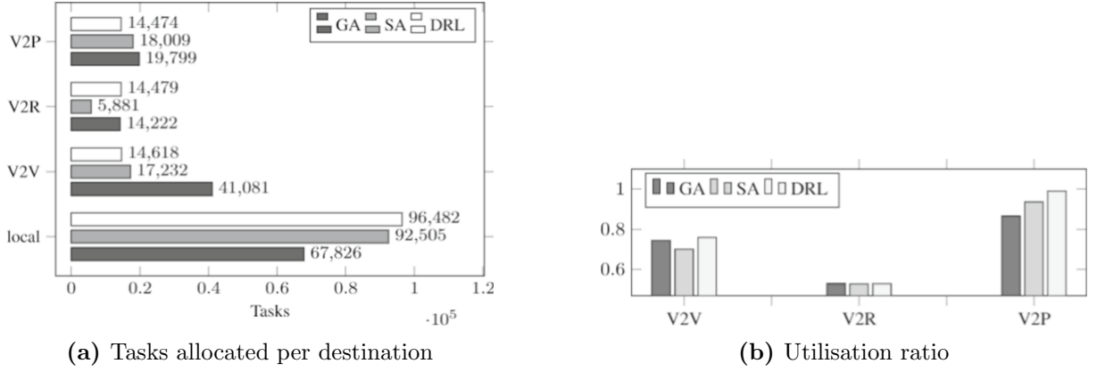
Figure 3.1.4: Workload distribution and utilisation ratio at \lambda = 200 tasks/s [1]
