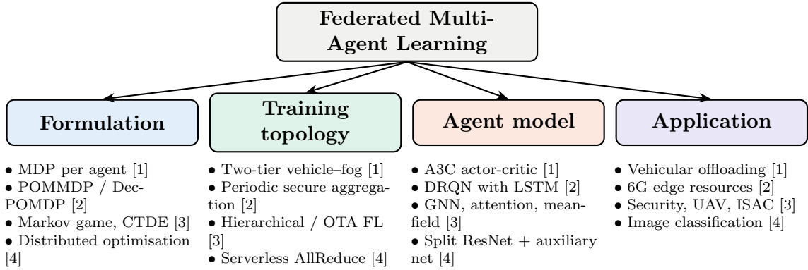
Figure 2.10.1: A taxonomy of federated multi-agent learning and the positions of the reviewed works
