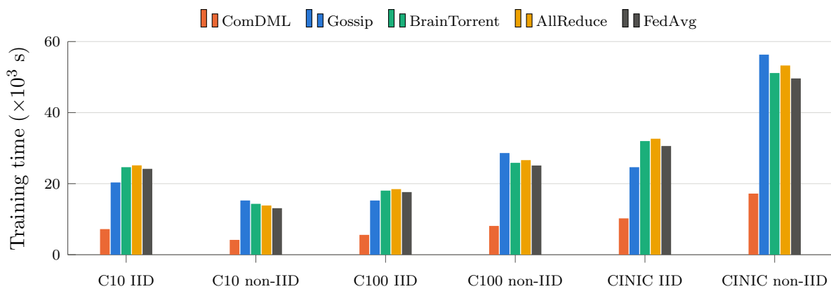
Figure 3.4.3: Training time to target accuracy with 10 heterogeneous agents, plotted from Table 3.4
