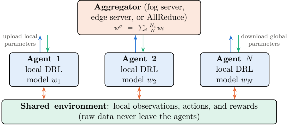
Figure 2.6.1: Federated multi-agent reinforcement learning: agents learn locally from their own interaction and periodically fuse model parameters through an aggregator
