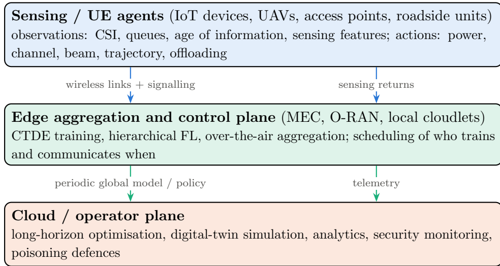
Figure 3.3.1: Conceptual architecture for distributed sensing, wireless communication, and multi-agent deep learning (redrawn from [3])
