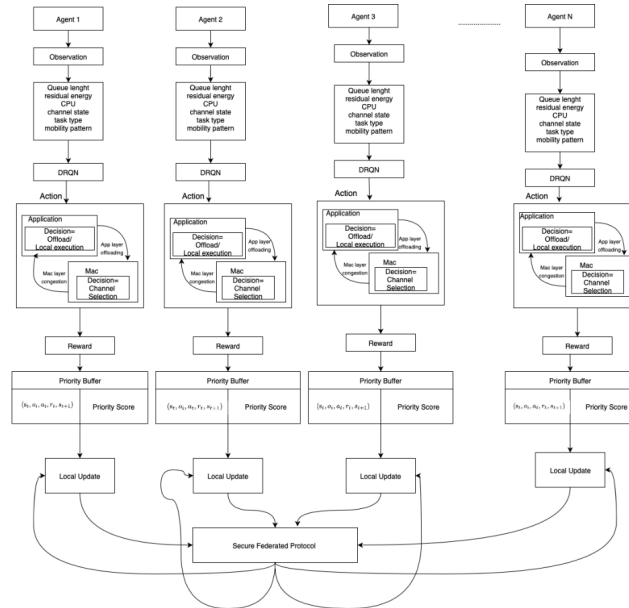
Figure 3.2.1: System architecture of FERMI-6G: each agent observes local state, selects application- and MAC-layer actions with a DRQN, stores prioritised experience, updates locally, and joins the secure federated protocol [2]
