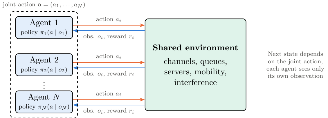
Figure 2.3.1: Multi-agent reinforcement learning under partial observability: every agent acts on local observations, but the environment responds to the joint action
