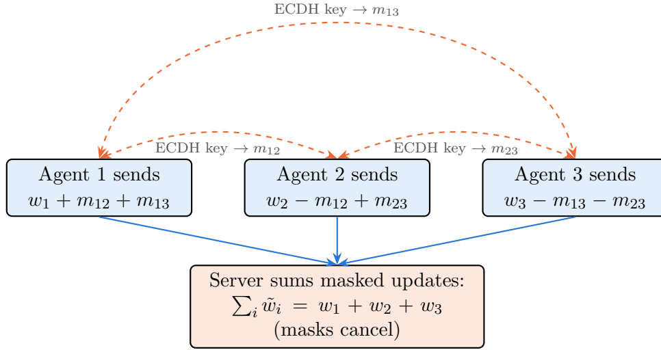
Figure 2.7.1: Secure aggregation with pairwise masks: each individual upload is hidden, but the masks cancel in the sum
