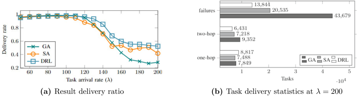
Figure 3.1.3: Delivery ratio versus arrival rate, and one-hop deliveries, two-hop deliveries, and failures at \lambda = 200 [1]
