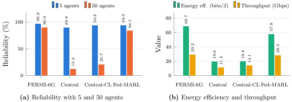
Figure 3.2.3: Scalability, energy efficiency, and throughput of the four frameworks, plotted from Table 3.1 (Central-CL: centralised RL with cross-layer optimisation)
