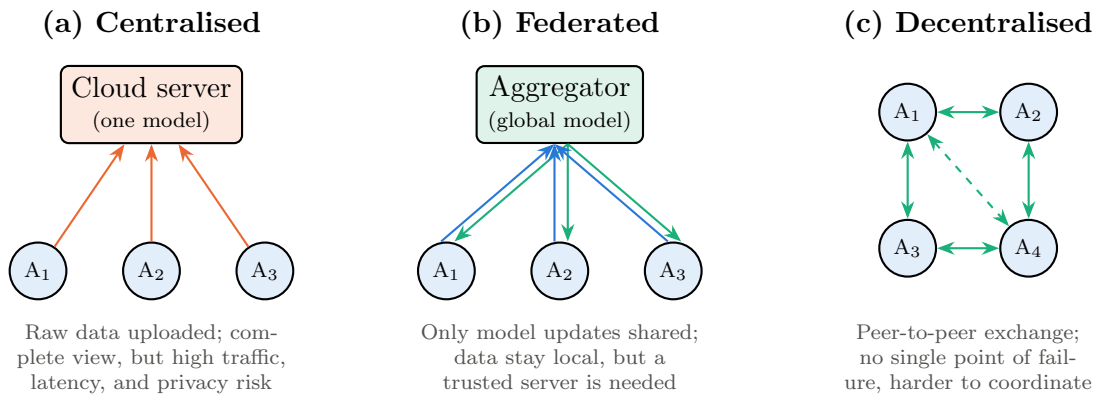
Figure 1.1.1: Three paradigms for learning across many agents: centralised, federated, and decentralised (peer-to-peer)
