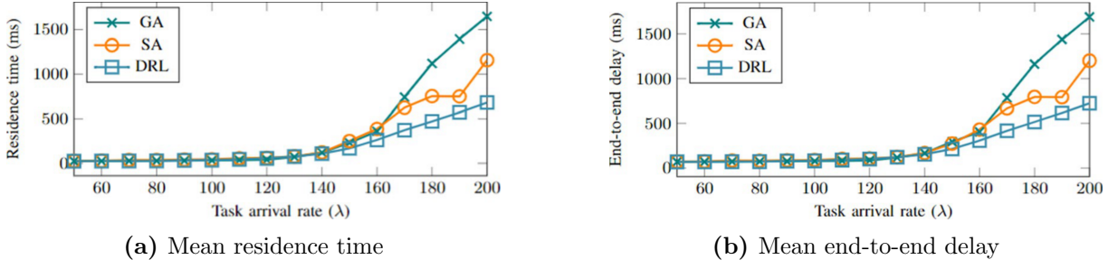
Figure 3.1.2: Residence time and end-to-end delay versus task arrival rate for GA, SA, and the proposed DRL scheme [1]
