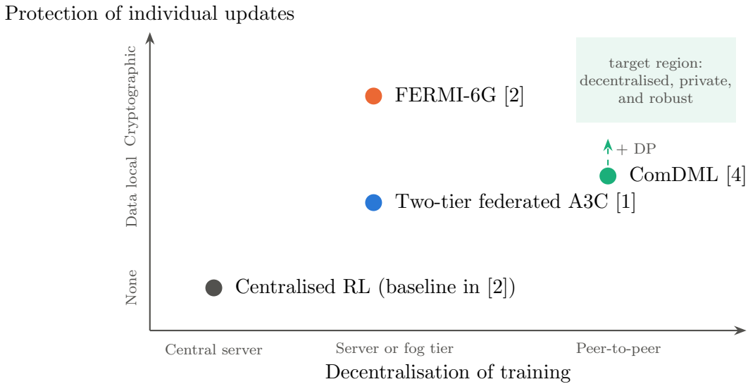
Figure 4.2.1: Qualitative design space of the reviewed systems: degree of decentralisation versus protection of individual model updates
