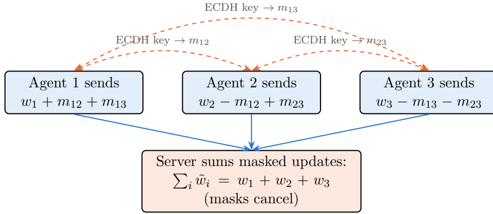
Figure 2.7.1: Secure aggregation with pairwise masks: each individual upload is hidden, but the masks cancel in the sum
