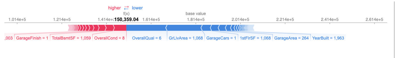
FIGURE 11. SHAP Force Plot for a House Price Prediction (XGBoost).
