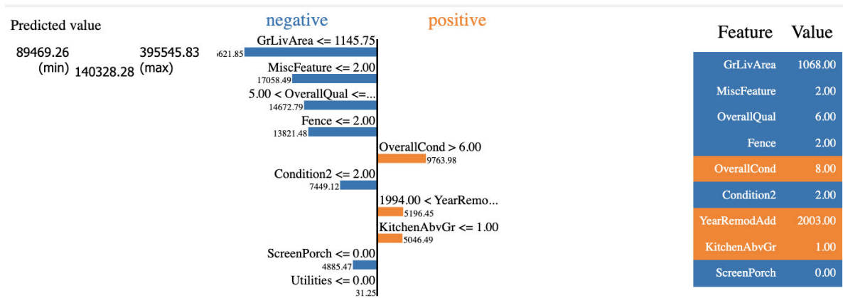
FIGURE 9. LIME Explanation for House Price Prediction using LightGBM.
