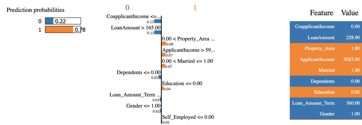
FIGURE 3. LIME Explanation for Loan Approval using LightGBM.
