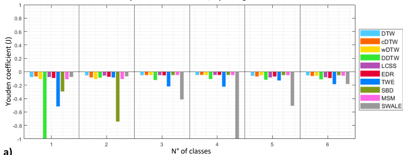
Synthetic Control dataset, equal lengths
