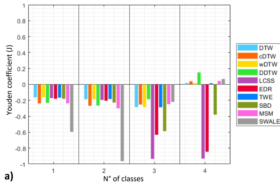
Trace dataset, equal lengths
