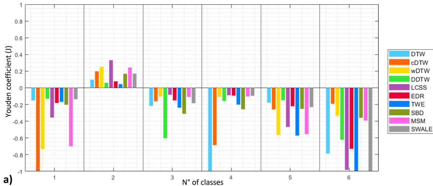
Lightning7 dataset, equal lengths
