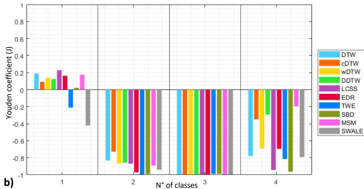
FaceFour dataset, variable lengths
