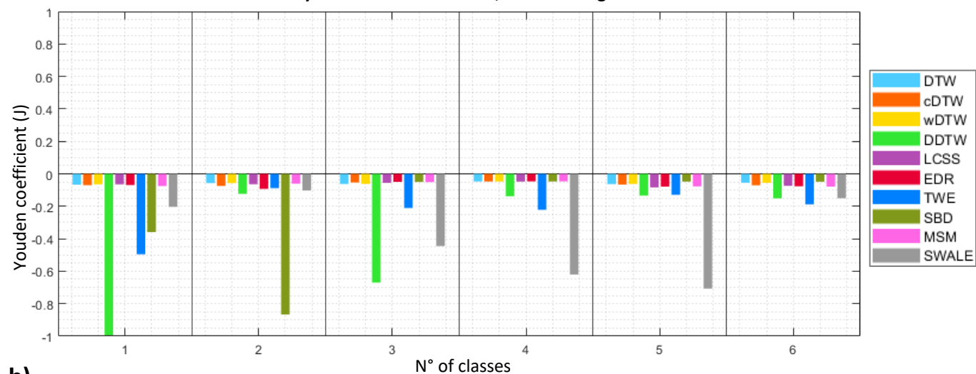
Synthetic Control dataset, variable lengths
