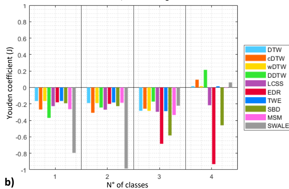
Trace dataset, variable lengths
