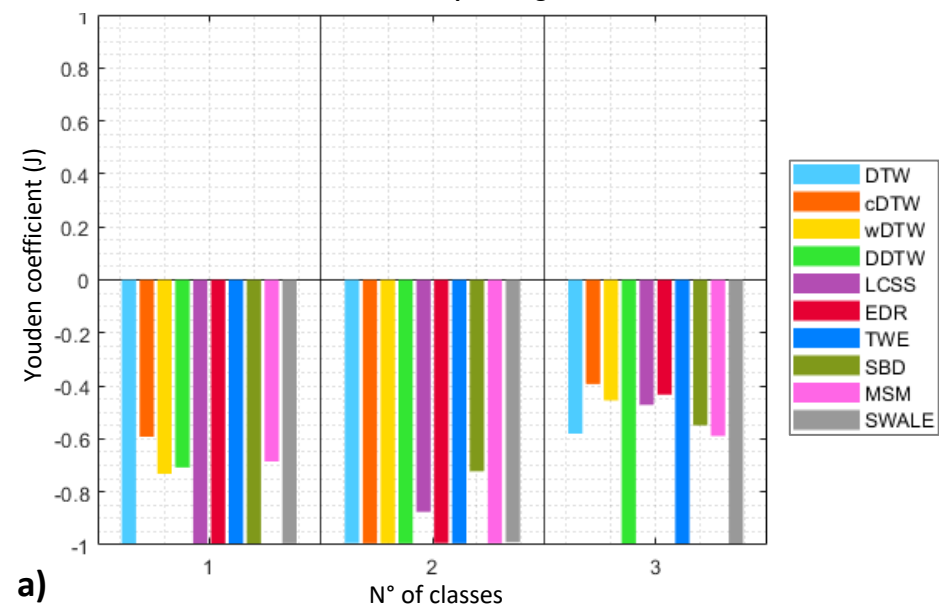
CBF dataset, equal lengths
