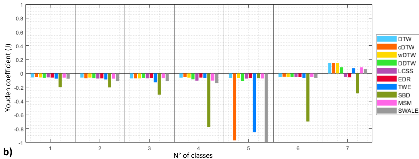
Plane dataset, variable lengths
