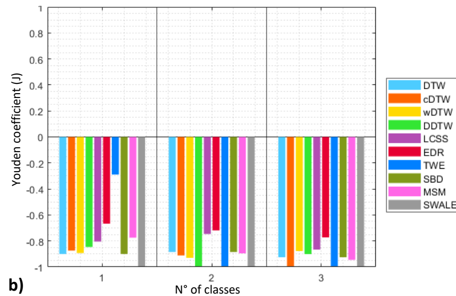
SmoothSubspace dataset, variable lengths
