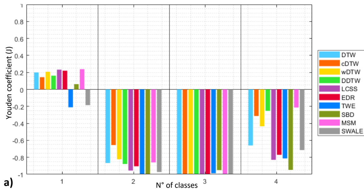
FaceFour dataset, equal lengths
