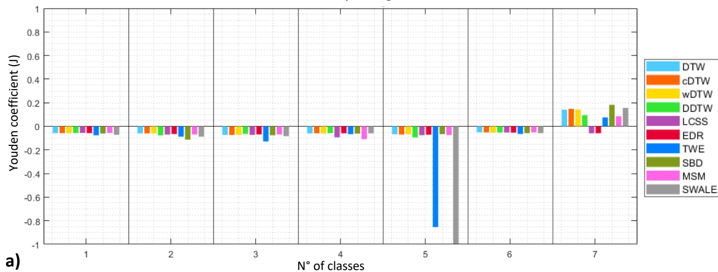
Plane dataset, equal lengths
