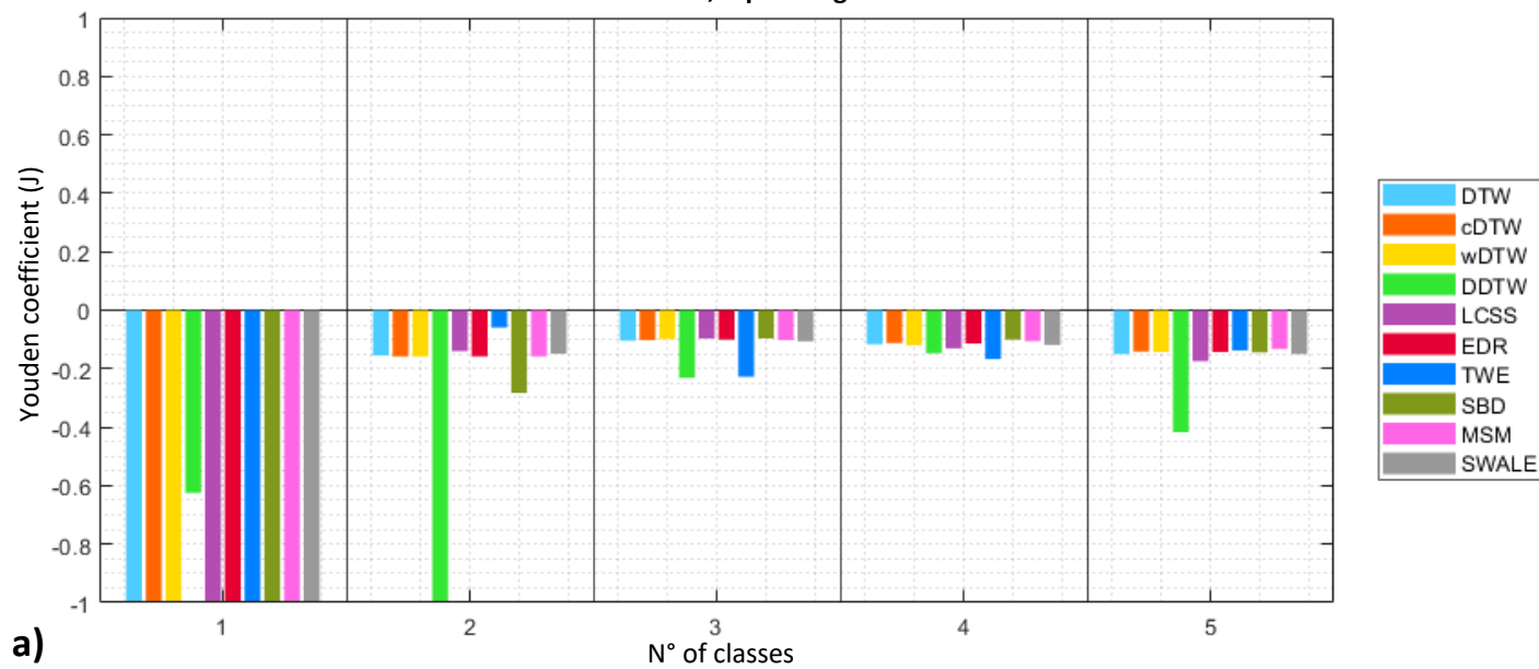
Beef dataset, equal lengths
