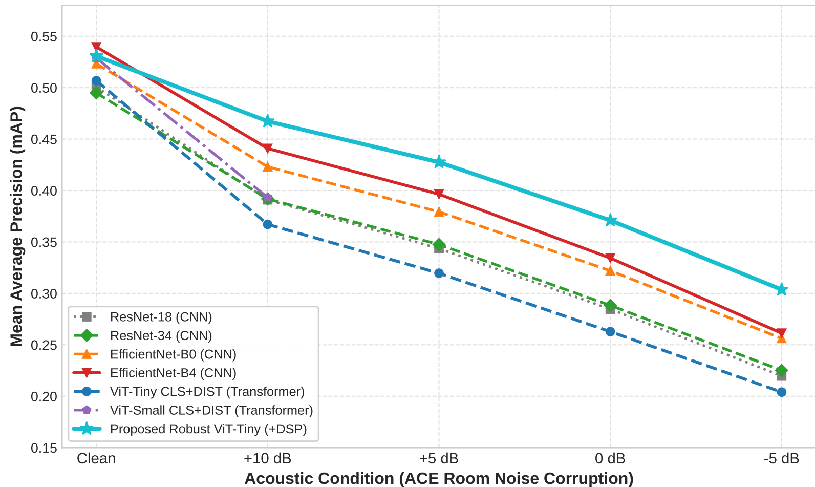
Cross-Architectural Noise Degradation Benchmark on Held-Out FSD50K
