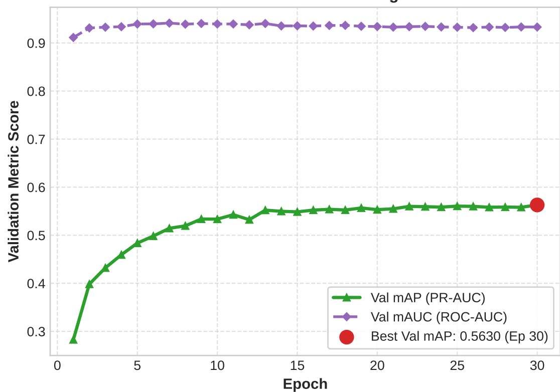
Validation mAP and mAUC Progression
