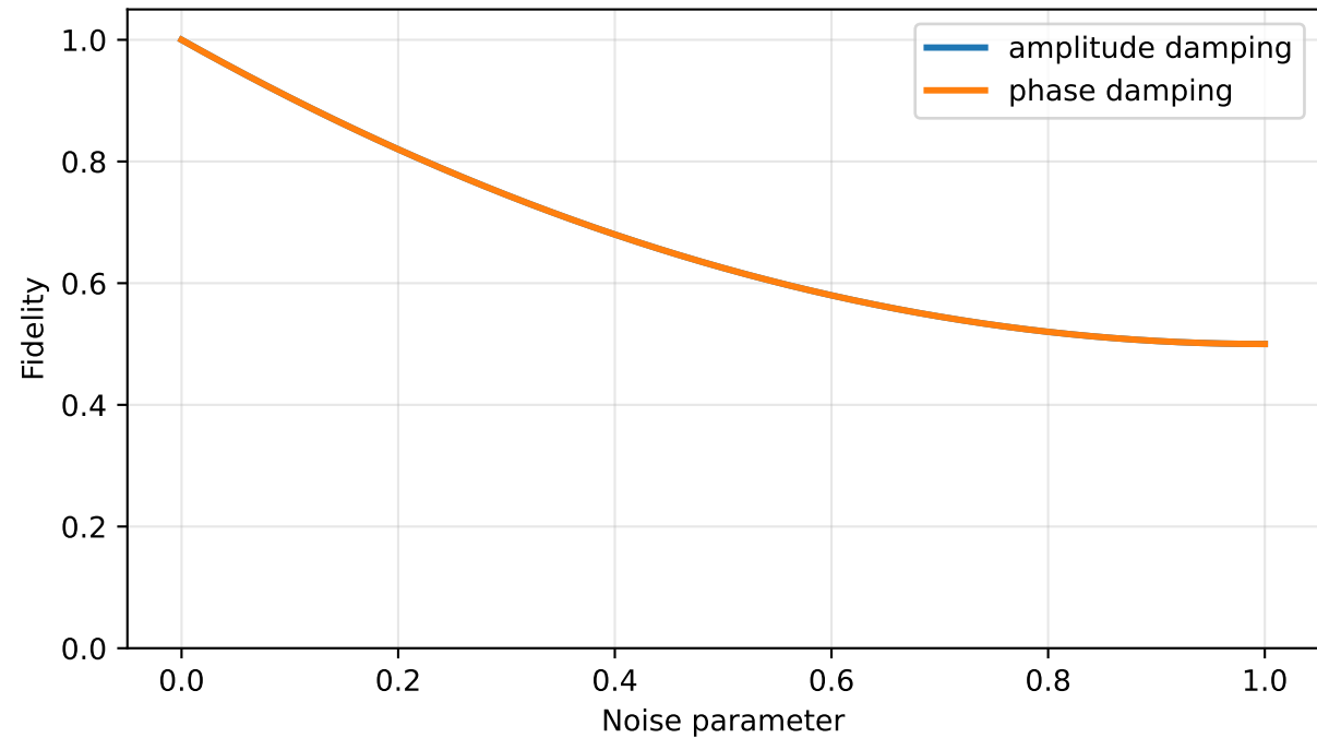
Bell-state fidelity under local noise
