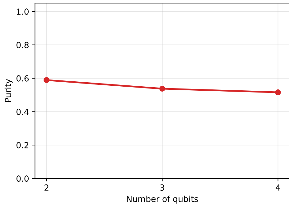
GHZ scaling under phase damping (noise=0.35)
