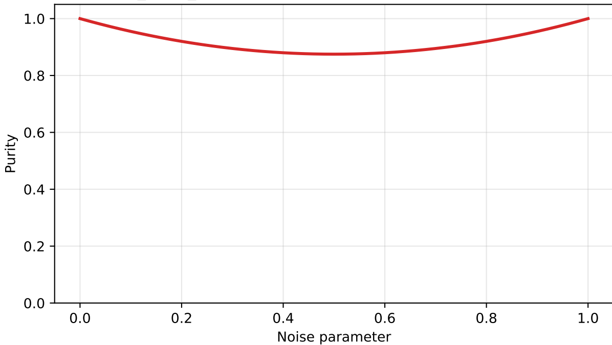
single_qubit_superposition purity under amplitude damping
