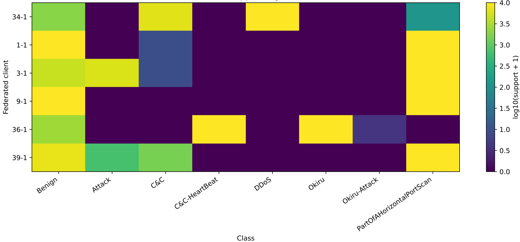
IoT-23 client/class support (log10 count + 1)
