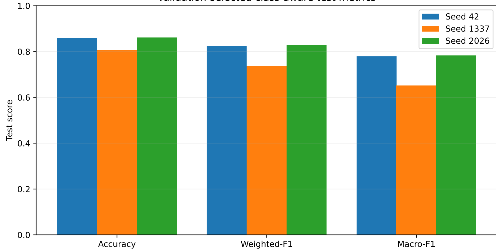
Validation-selected class-aware test metrics
