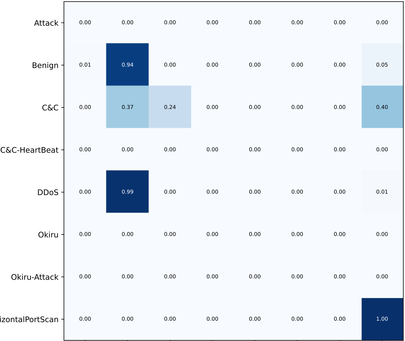
Confusion matrix hardest LOSO 34-1 — normalized by true class (seed 42)
