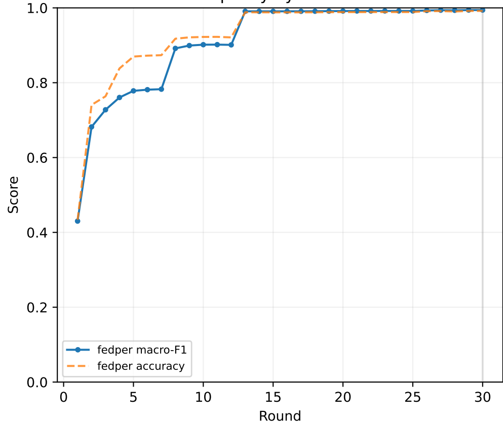
Validation quality by federated round
