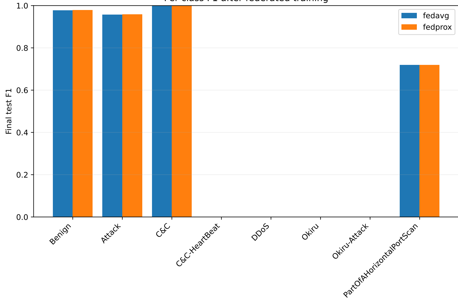
Per-class F1 after federated training
